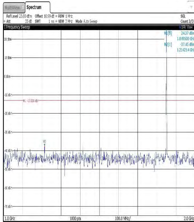
Band2-1.4MHz-QPSK-18607-1RB#0-Range2:1000~2000MHz
