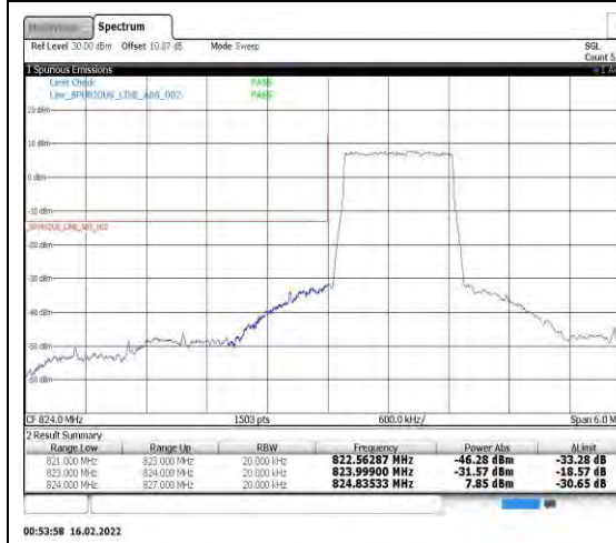
Band26-1.4MHz-QPSK-26797-6RB#0
