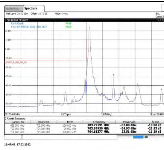
Band17-10MHz-QPSK-23780-1RB#0
