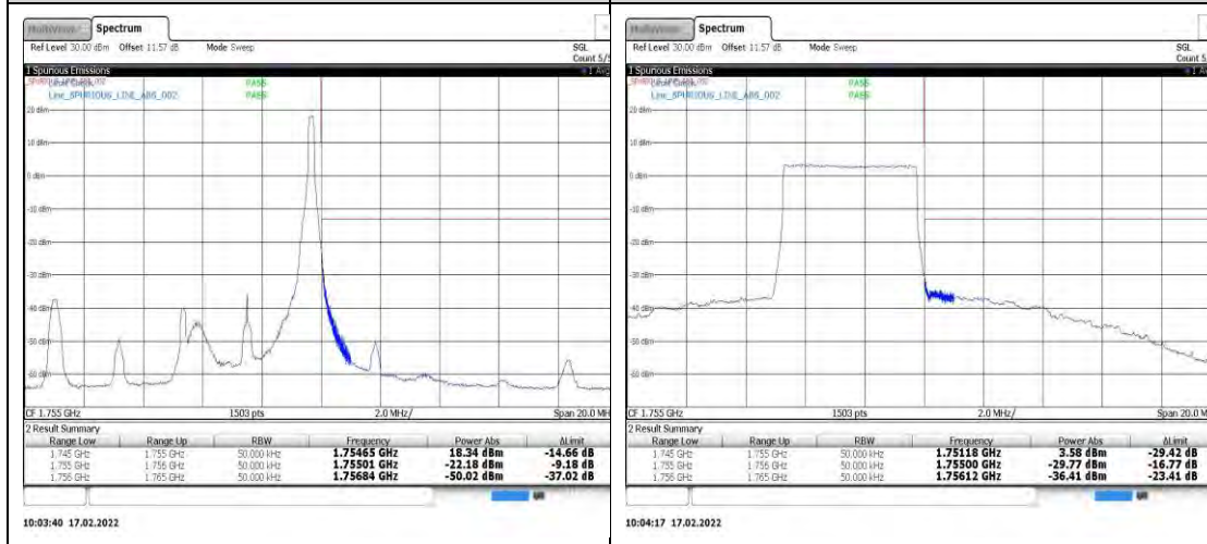
Band4-5MHz-16QAM-20375-1RB#24
