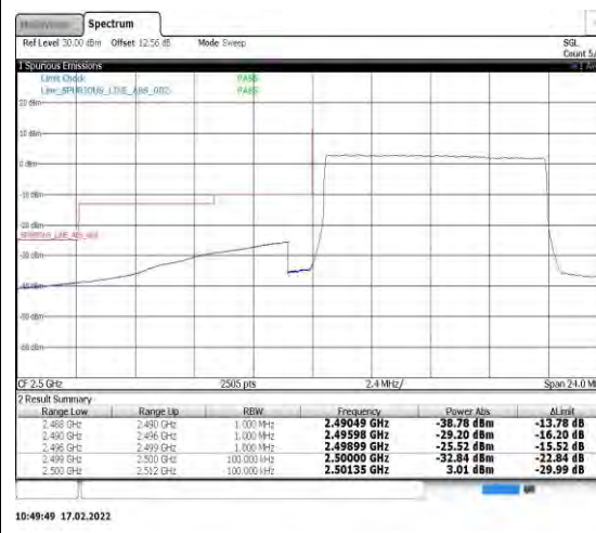
Band7-10MHz-16QAM-20800-50RB#0
