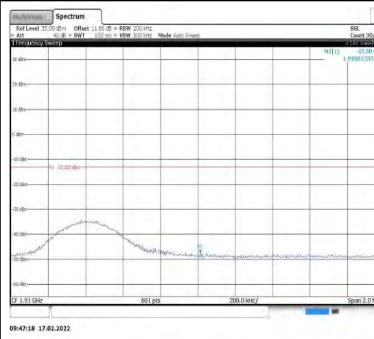
Band2-10MHz-16QAM-19150-1RB#0
