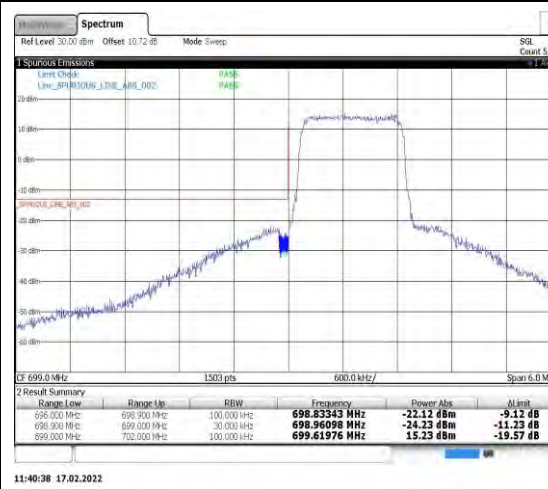
Band12-1.4MHz-16QAM-23017-6RB#0
