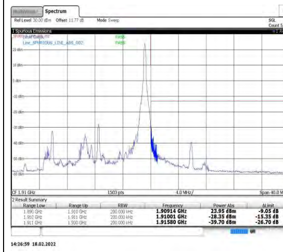
Band2-15MHz-QPSK-19125-1RB#74
