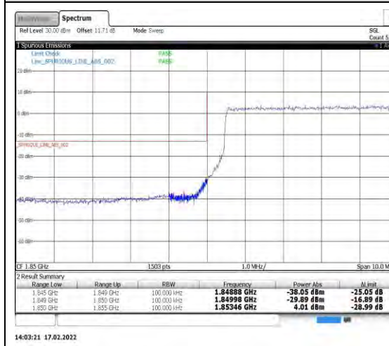
Band25-10MHz-QPSK-26090-50RB#0
