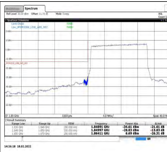
Band2-15MHz-QPSK-18675-75RB#0
