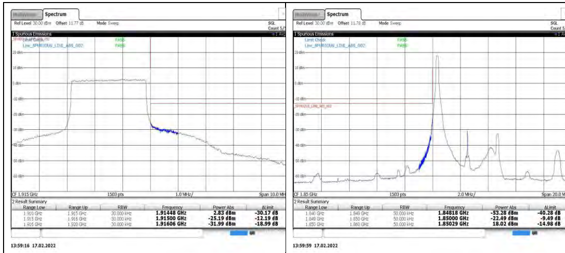
Band25-3MHz-16QAM-26675-15RB#0
