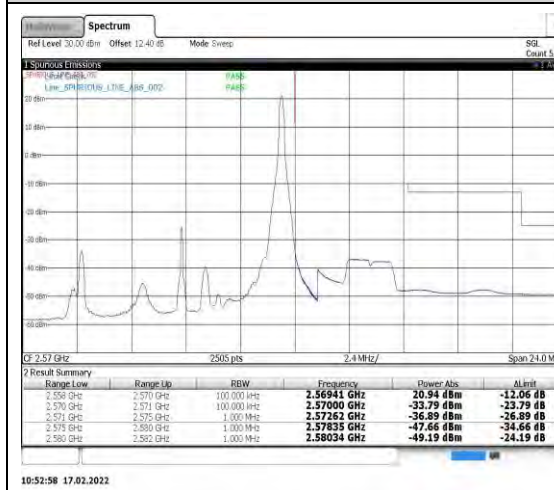
Band7-10MHz-16QAM-21400-1RB#49
