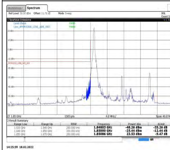
Band2-15MHz-16QAM-18675-1RB#0
