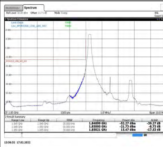
Band25-3MHz-16QAM-26055-1RB#0
