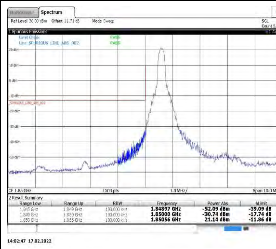
Band25-10MHz-QPSK-26090-1RB#0
