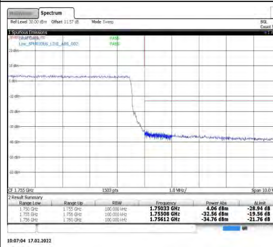
Band4-10MHz-16QAM-20350-50RB#0
