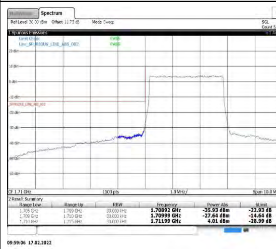
Band4-3MHz-16QAM-19965-15RB#0
