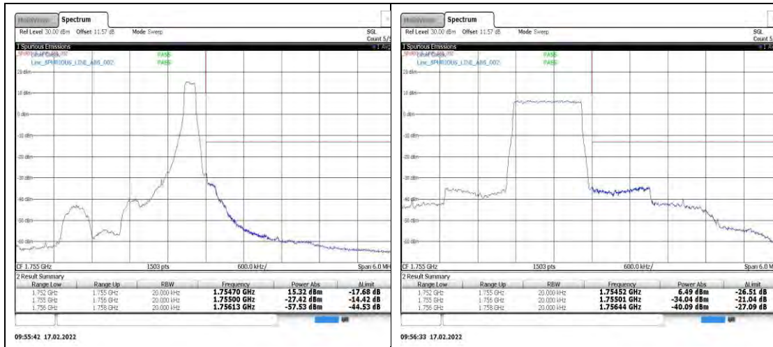
Band4-1.4MHz-QPSK-20393-1RB#5
