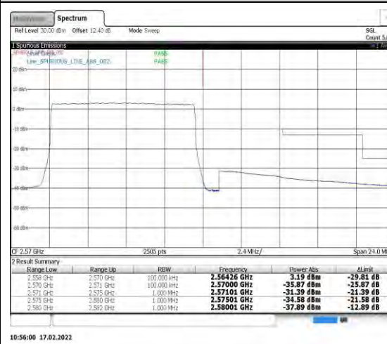
Band7-10MHz-16QAM-21400-50RB#0
