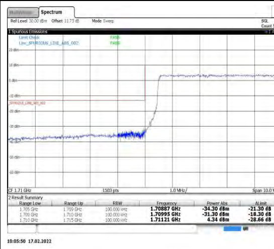
Band4-10MHz-16QAM-20000-50RB#0
