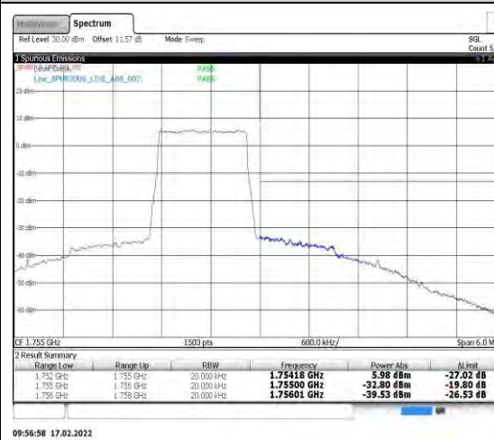
Band4-1.4MHz-16QAM-20393-6RB#0
