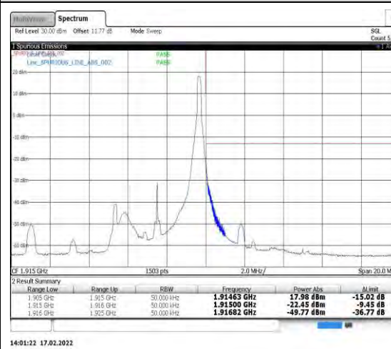
Band25-5MHz-QPSK-26665-1RB#24
