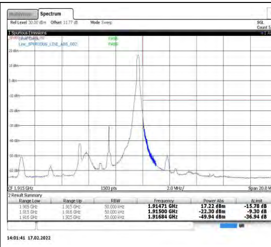
Band25-5MHz-16QAM-26665-1RB#24
