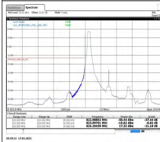
Band5-3MHz-16QAM-20415-1RB#0
