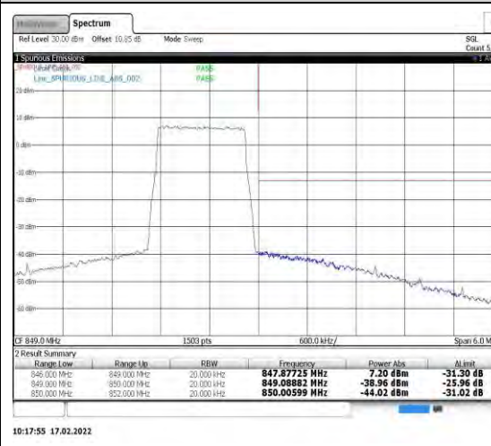
Band5-1.4MHz-16QAM-20643-6RB#0
