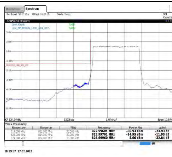
Band5-3MHz-QPSK-20415-15RB#0
