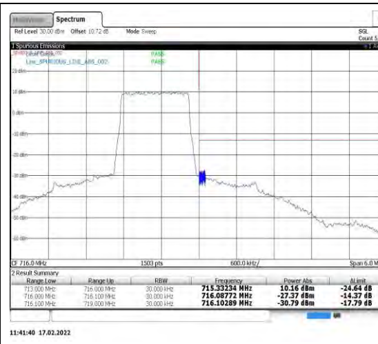
Band12-1.4MHz-QPSK-23173-6RB#0
