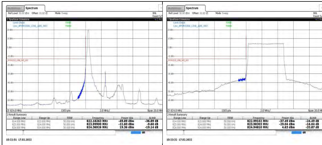
Band5-5MHz-16QAM-20425-1RB#0
