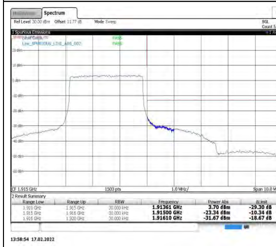
Band25-3MHz-QPSK-26675-15RB#0
