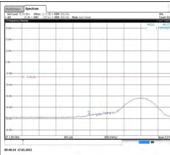
Band2-10MHz-16QAM-18650-1RB#49
