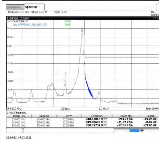
Band5-5MHz-16QAM-20625-1RB#24
