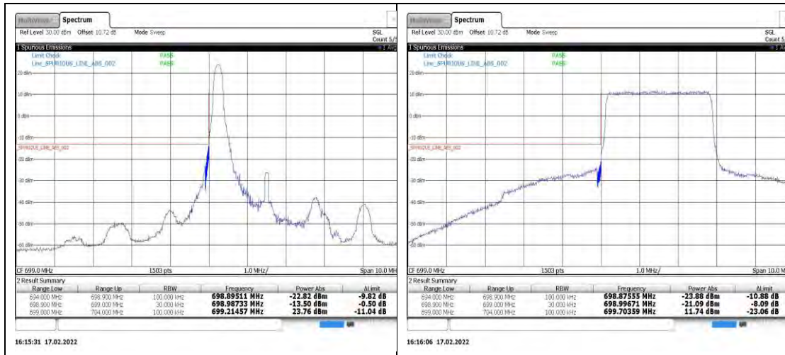
Band12-3MHz-QPSK-23025-1RB#0
