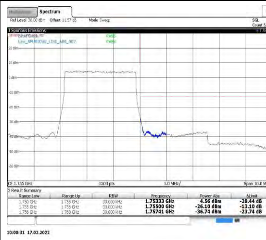
Band4-3MHz-QPSK-20385-15RB#0
