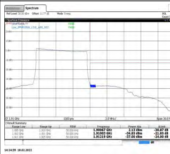
Band2-10MHz-16QAM-19150-50RB#0
