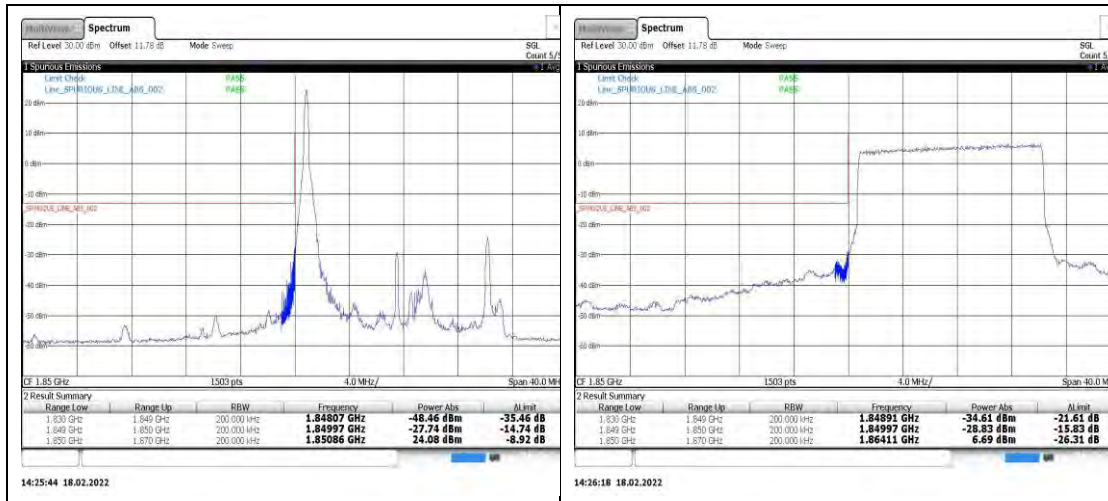
Band2-15MHz-QPSK-18675-1RB#0
