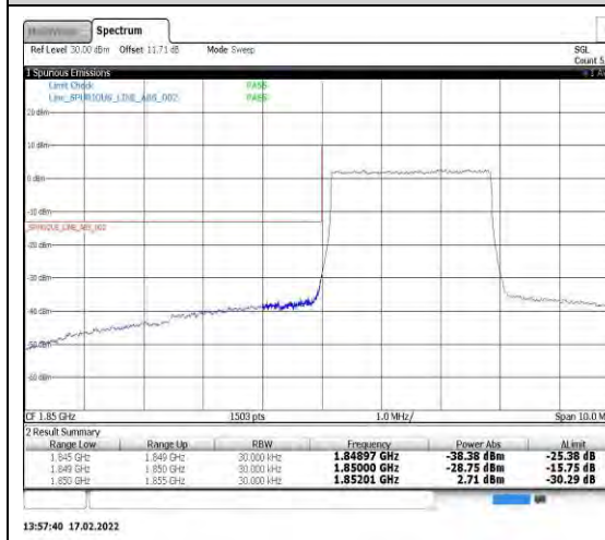
Band25-3MHz-16QAM-26055-15RB#0
