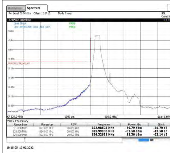
Band5-1.4MHz-16QAM-20407-1RB#0
