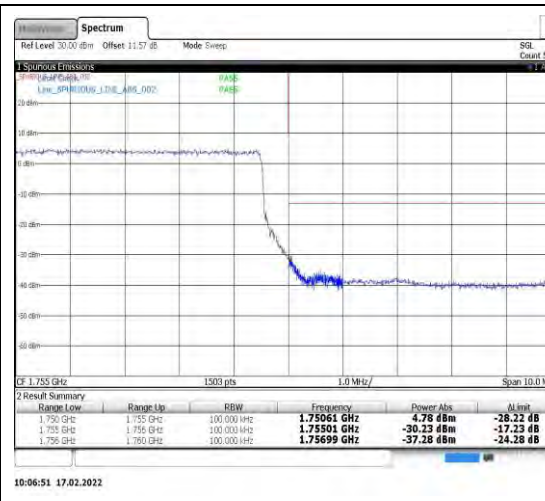
Band4-10MHz-QPSK-20350-50RB#0
