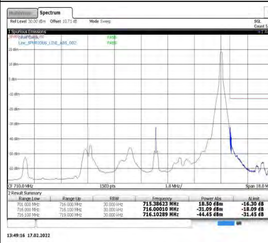
Band17-10MHz-QPSK-23800-1RB#49
