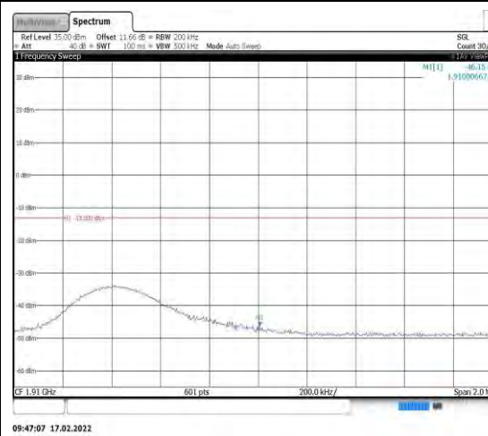
Band2-10MHz-QPSK-19150-1RB#0
