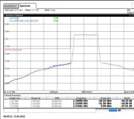
Band4-1.4MHz-16QAM-19957-6RB#0
