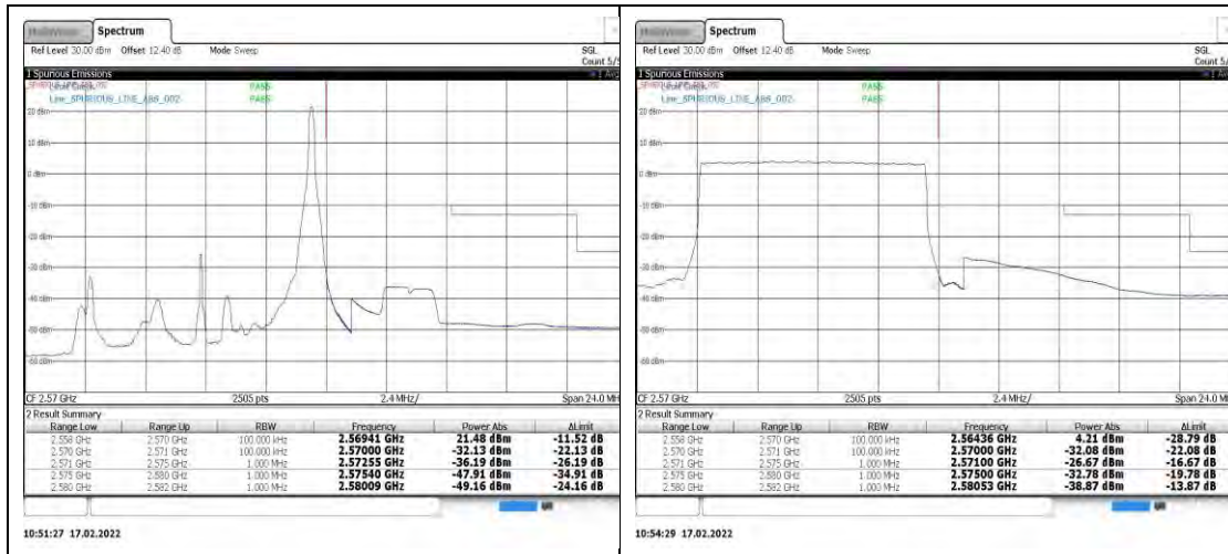
Band7-10MHz-QPSK-21400-1RB#49
