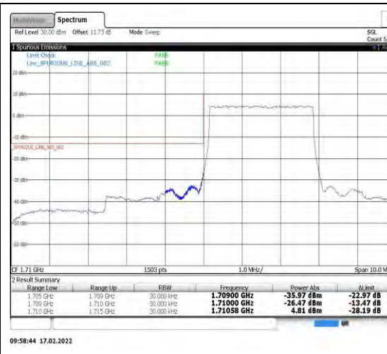
Band4-3MHz-QPSK-19965-15RB#0
