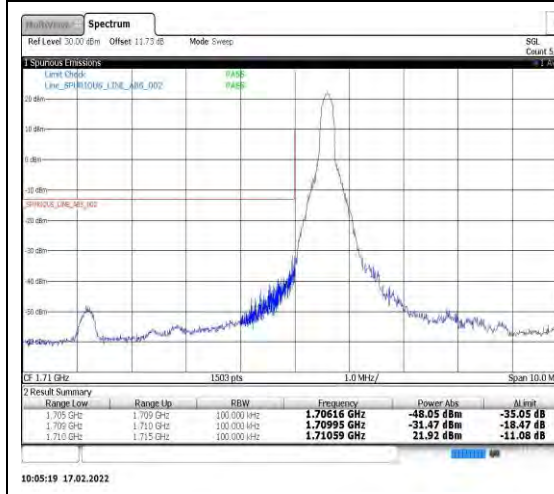
Band4-10MHz-16QAM-20000-1RB#0
