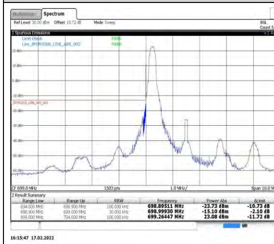
Band12-3MHz-16QAM-23025-1RB#0
