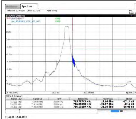
Band12-1.4MHz-16QAM-23173-1RB#5
