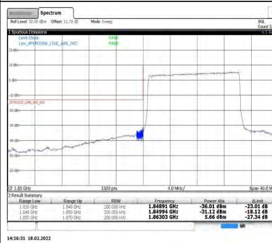
Band2-15MHz-16QAM-18675-75RB#0
