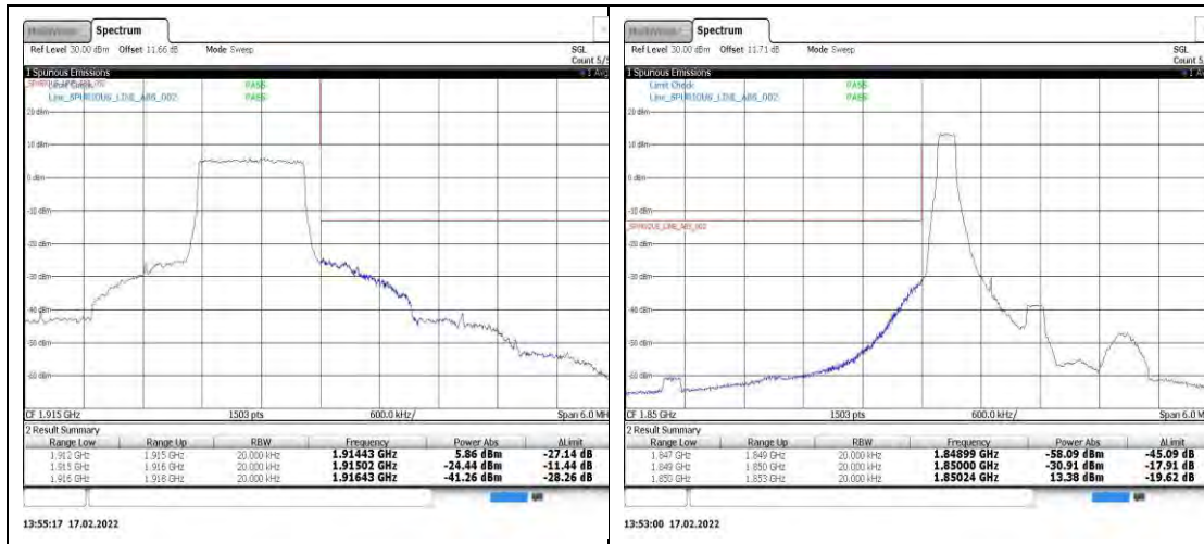
Band25-1.4MHz-QPSK-26683-6RB#0
