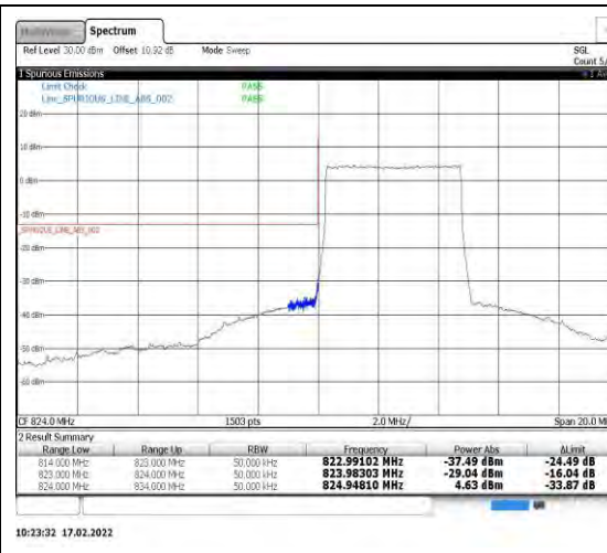
Band5-5MHz-16QAM-20425-25RB#0
