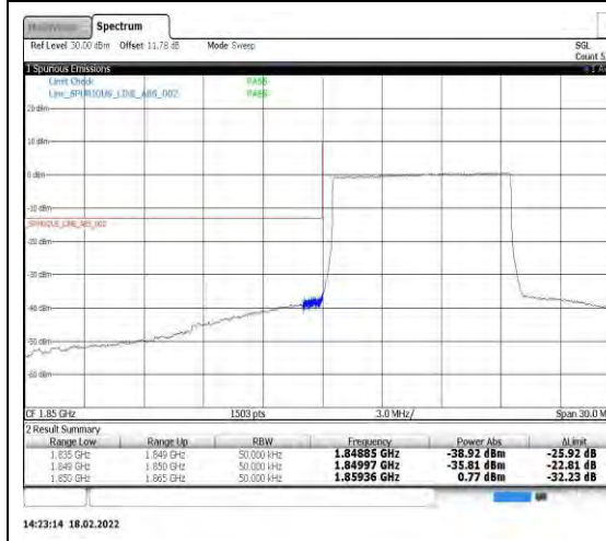
Band2-10MHz-16QAM-18650-50RB#0
