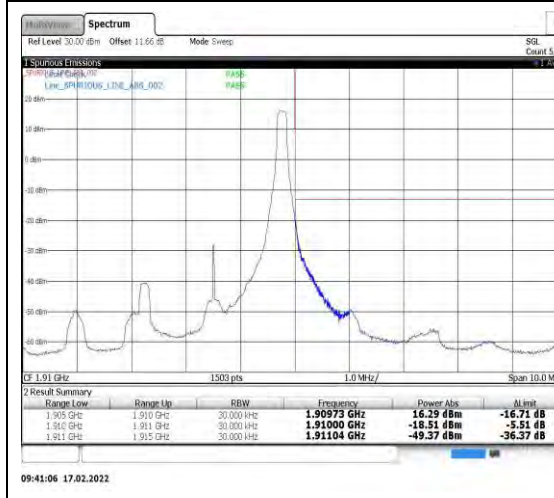
Band2-3MHz-16QAM-19185-1RB#14
