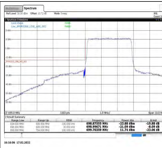
Band12-3MHz-QPSK-23025-15RB#0
