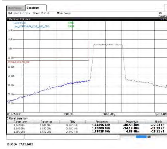
Band25-1.4MHz-16QAM-26047-6RB#0
