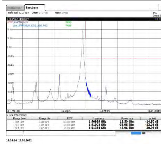
Band2-10MHz-16QAM-19150-1RB#49
