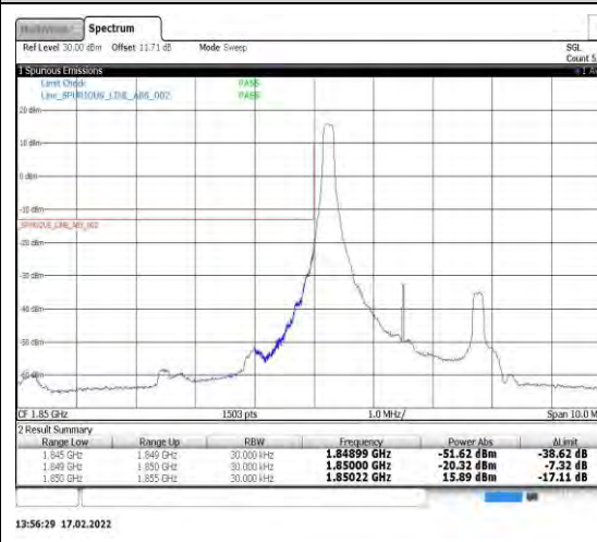
Band25-3MHz-QPSK-26055-1RB#0
