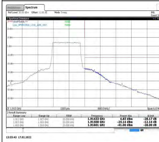
Band25-1.4MHz-16QAM-26683-6RB#0
