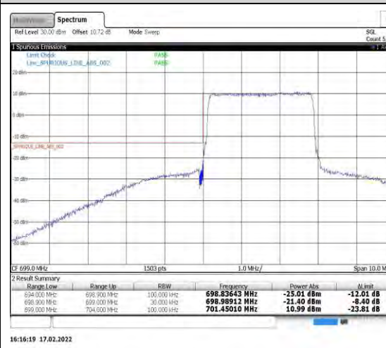
Band12-3MHz-16QAM-23025-15RB#0
