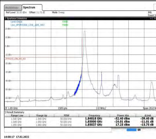
Band25-5MHz-16QAM-26065-1RB#0
