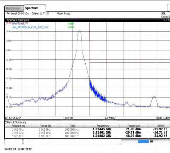
Band25-10MHz-QPSK-26640-1RB#49
