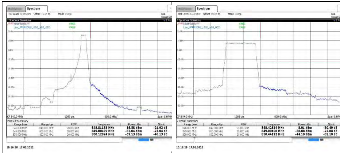
Band5-1.4MHz-QPSK-20643-1RB#5
