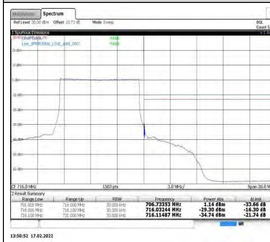
Band17-10MHz-QPSK-23800-50RB#0
