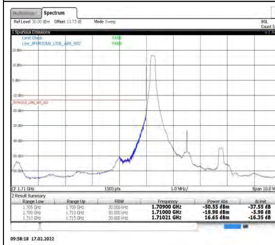
Band4-3MHz-16QAM-19965-1RB#0
