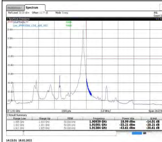
Band2-10MHz-QPSK-19150-1RB#49
