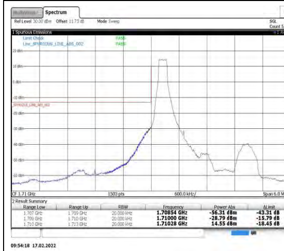
Band4-1.4MHz-16QAM-19957-1RB#0
