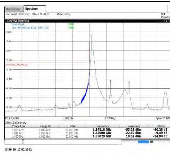
Band25-5MHz-QPSK-26065-1RB#0
