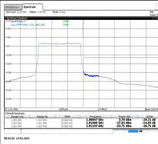
Band2-3MHz-16QAM-19185-15RB#0
