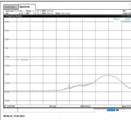
Band2-10MHz-QPSK-18650-1RB#49
