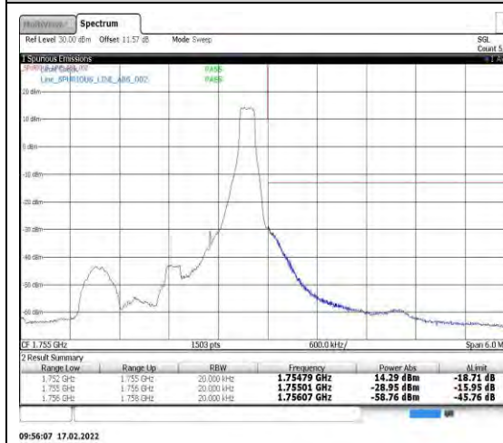
Band4-1.4MHz-16QAM-20393-1RB#5
