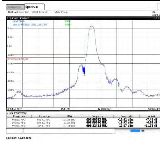
Band12-1.4MHz-16QAM-23017-1RB#0
