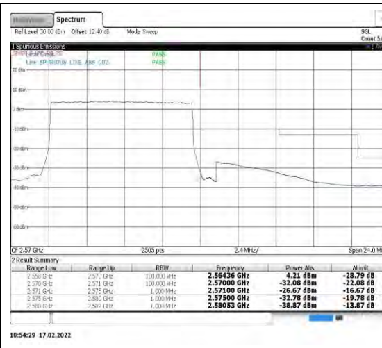
Band7-10MHz-QPSK-21400-50RB#0
