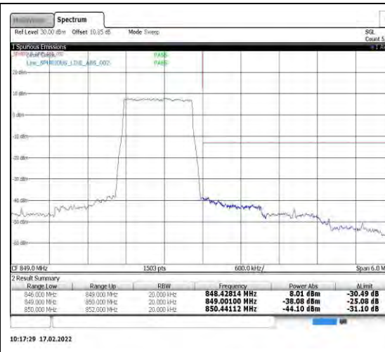
Band5-1.4MHz-QPSK-20643-6RB#0
