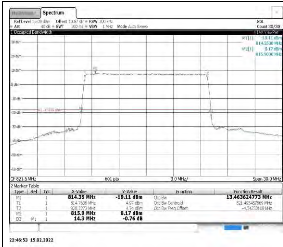
Band26-15MHz-16QAM-26765-75RB#0
