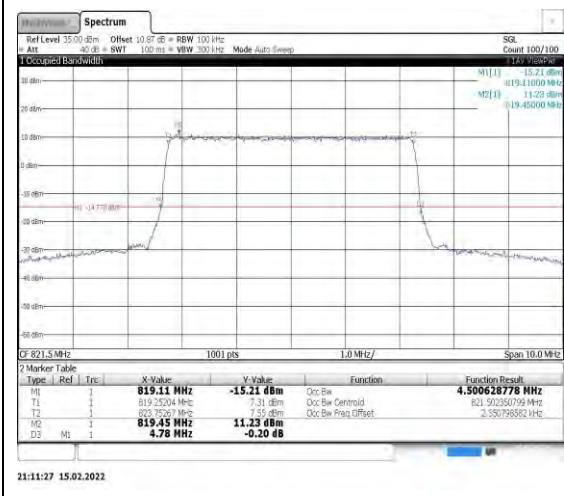
Band26-5MHz-QPSK-26765-25RB#0
