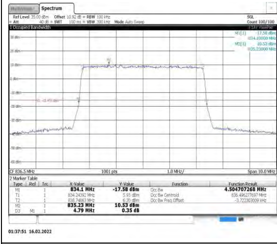
Band26-5MHz-16QAM-26915-25RB#0
