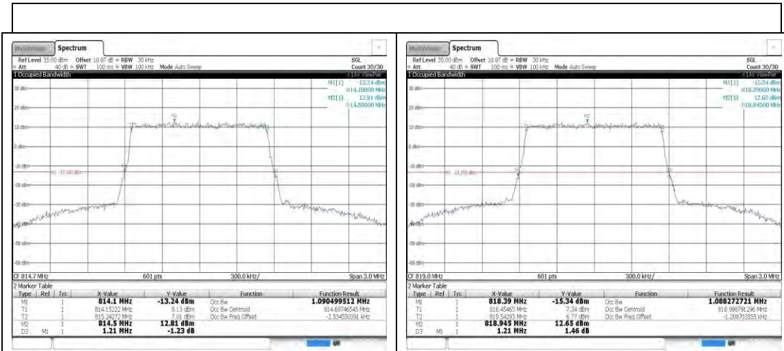
Band26-1.4MHz-QPSK-26697-6RB#0
