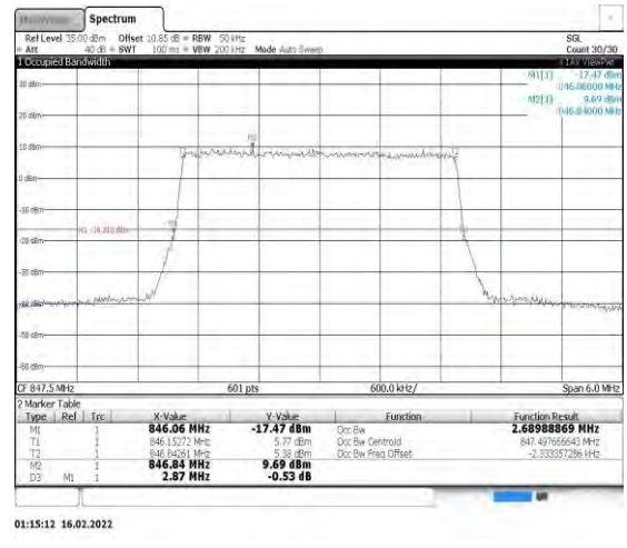
Band26-3MHz-16QAM-27025-15RB#0
