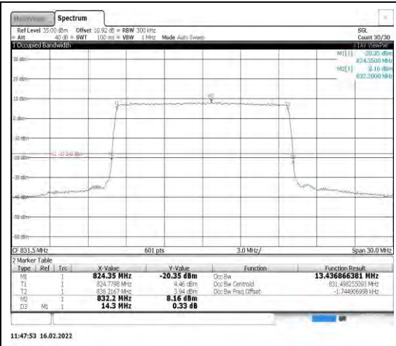
Band26-15MHz-16QAM-26865-75RB#0
