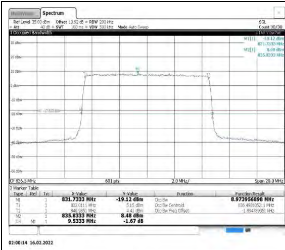
Band26-10MHz-16QAM-26915-50RB#0
