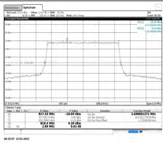
Band26-3MHz-16QAM-26740-15RB#0
