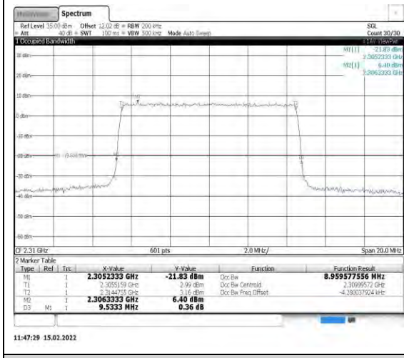
Band40-10MHz-16QAM-38750-50RB#0
