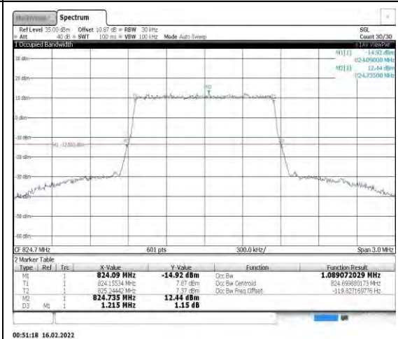
Band26-1.4MHz-QPSK-26797-6RB#0
