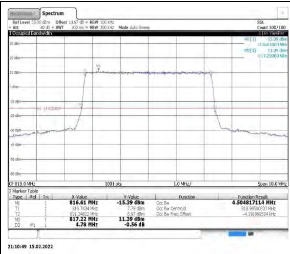
Band26-5MHz-QPSK-26740-25RB#0
