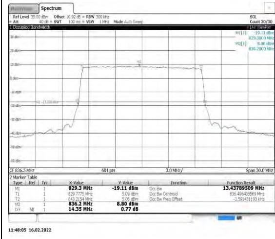
Band26-15MHz-QPSK-26915-75RB#0
