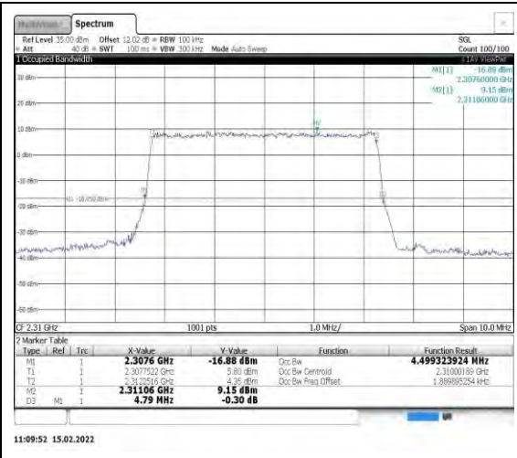
Band40-5MHz-QPSK-38750-25RB#0
