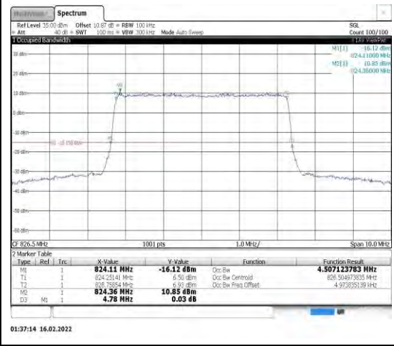
Band26-5MHz-16QAM-26815-25RB#0
