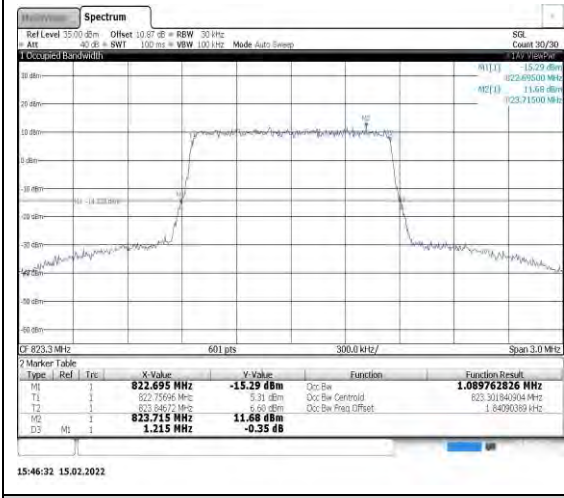
Band26-1.4MHz-16QAM-26783-6RB#0
