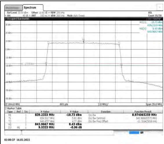
Band26-10MHz-16QAM-26990-50RB#0
