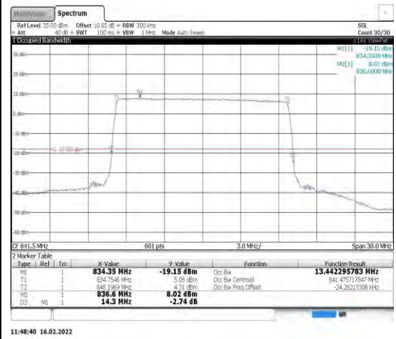
Band26-15MHz-16QAM-26965-75RB#0
