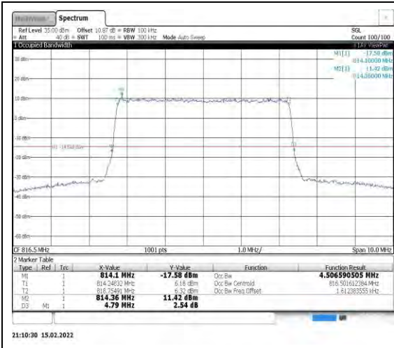
Band26-5MHz-16QAM-26715-25RB#0
