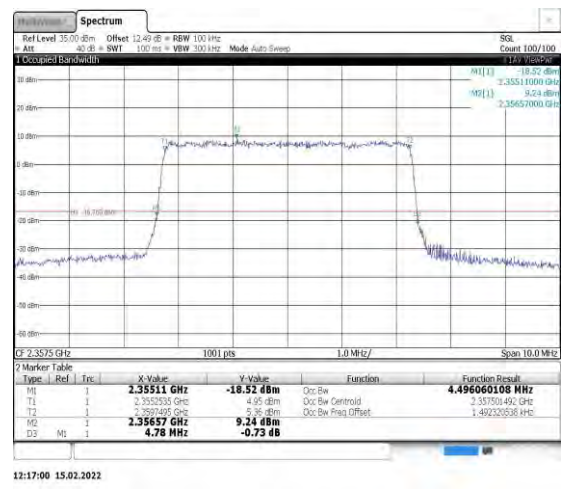
Band40-5MHz-16QAM-39225-25RB#0
