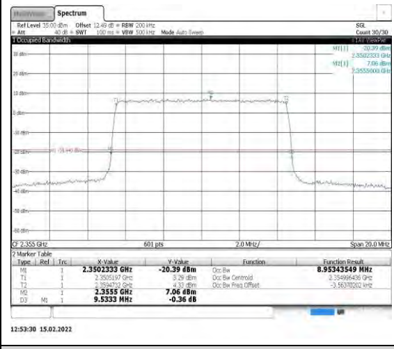
Band40-10MHz-16QAM-39200-50RB#0
