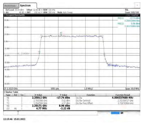
Band40-5MHz-16QAM-39175-25RB#0
