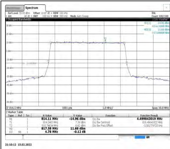
Band26-5MHz-QPSK-26715-25RB#0
