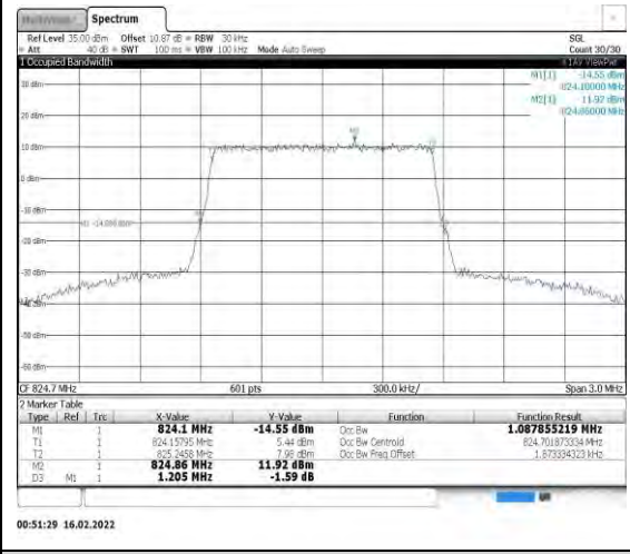
Band26-1.4MHz-16QAM-26797-6RB#0
