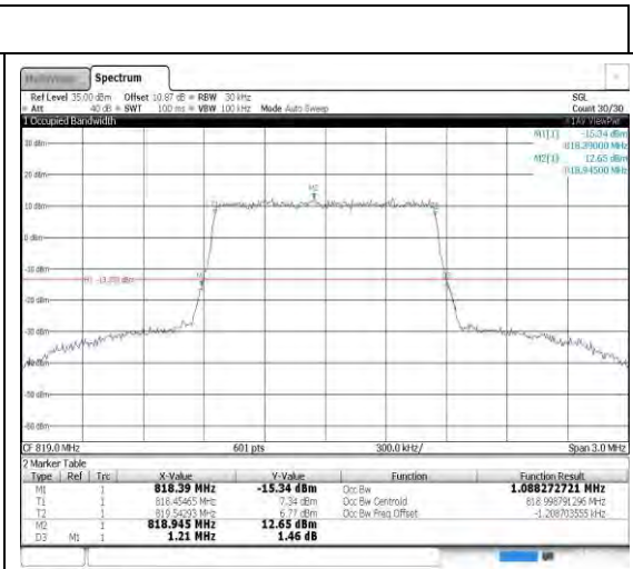
Band26-1.4MHz-QPSK-26740-6RB#0
