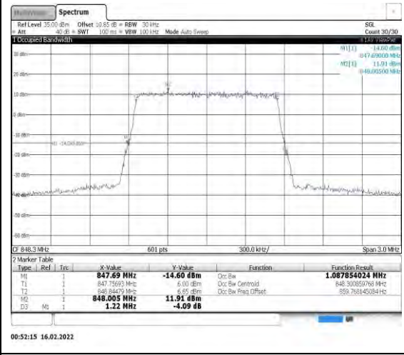
Band26-1.4MHz-16QAM-27033-6RB#0
