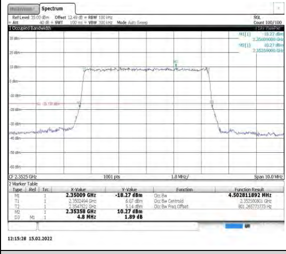
Band40-5MHz-QPSK-39175-25RB#0
