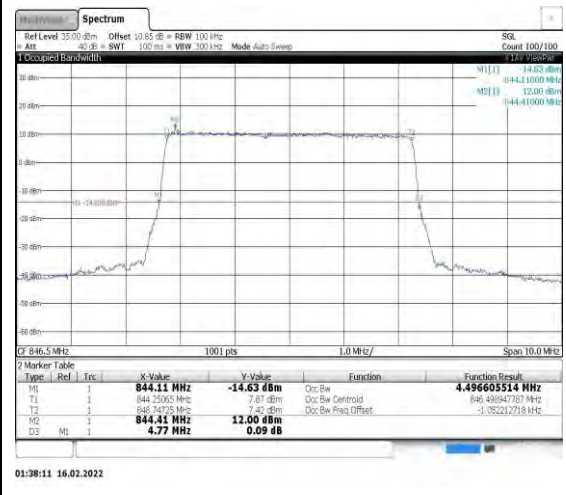
Band26-5MHz-QPSK-27015-25RB#0
