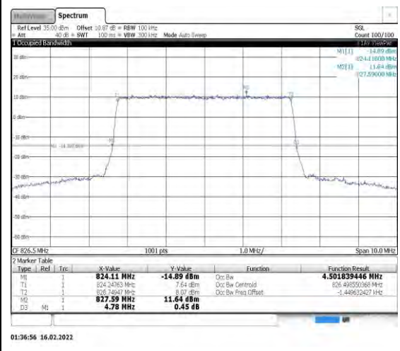
Band26-5MHz-QPSK-26815-25RB#0
