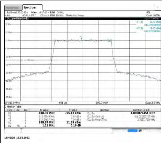
Band26-1.4MHz-16QAM-26740-6RB#0
