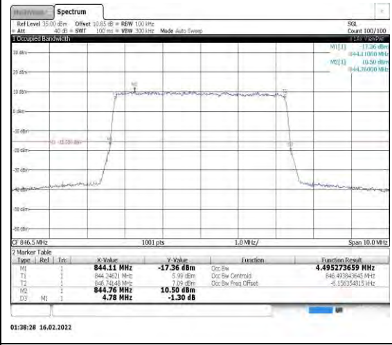
Band26-5MHz-16QAM-27015-25RB#0
