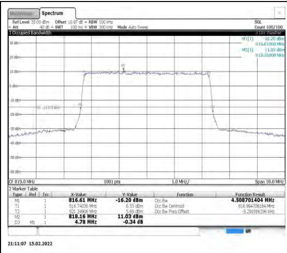
Band26-5MHz-16QAM-26740-25RB#0
