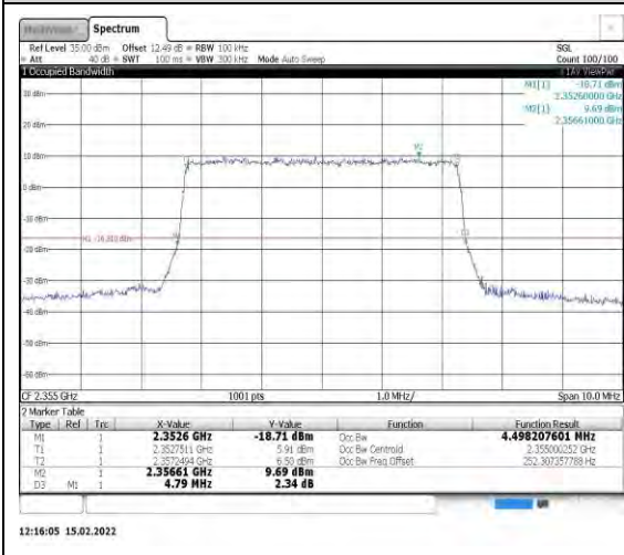
Band40-5MHz-QPSK-39200-25RB#0
