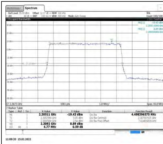
Band40-5MHz-16QAM-38725-25RB#0
