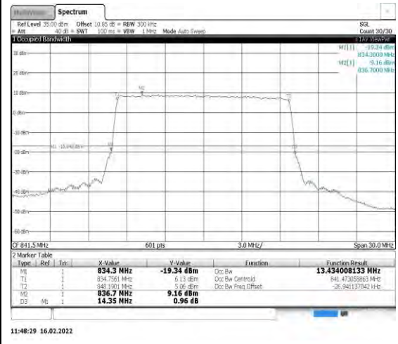
Band26-15MHz-QPSK-26965-75RB#0
