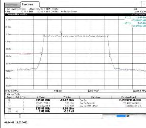
Band26-3MHz-16QAM-26915-15RB#0
