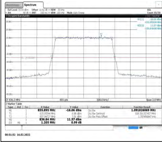
Band26-1.4MHz-16QAM-26915-6RB#0
