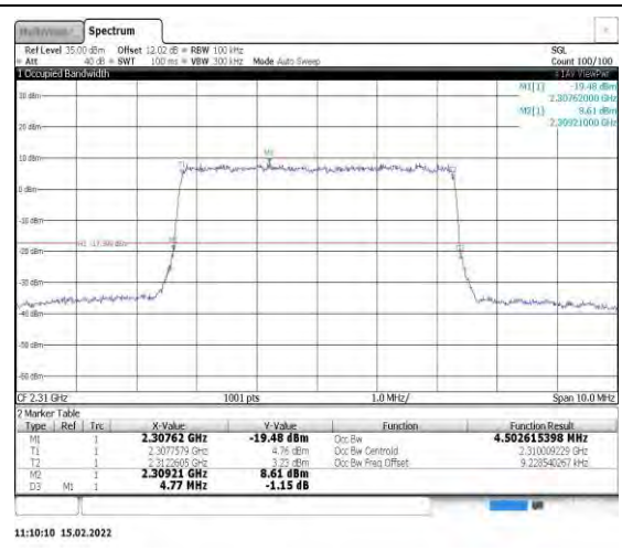
Band40-5MHz-16QAM-38750-25RB#0
