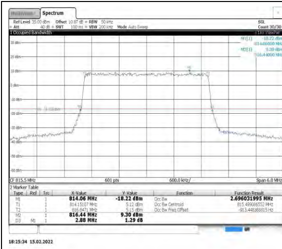
Band26-3MHz-16QAM-26705-15RB#0
