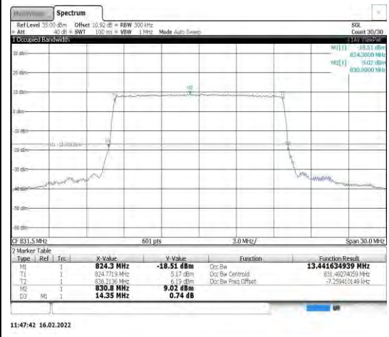
Band26-15MHz-QPSK-26865-75RB#0
