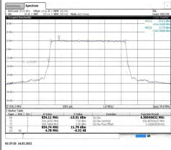
Band26-5MHz-QPSK-26915-25RB#0
