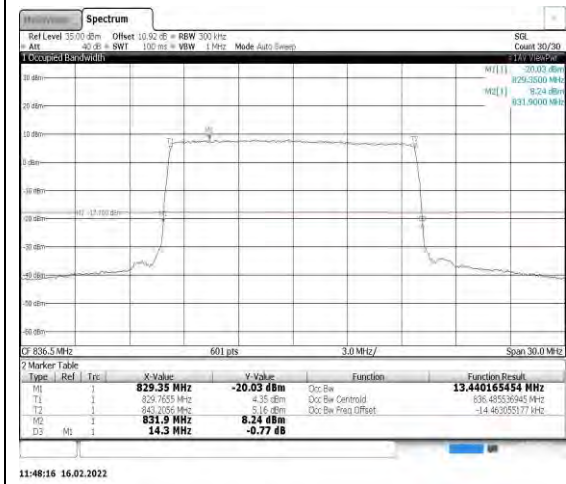
Band26-15MHz-16QAM-26915-75RB#0
