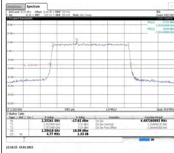
Band40-5MHz-16QAM-39200-25RB#0
