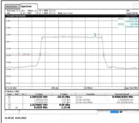
Band40-10MHz-QPSK-38750-50RB#0
