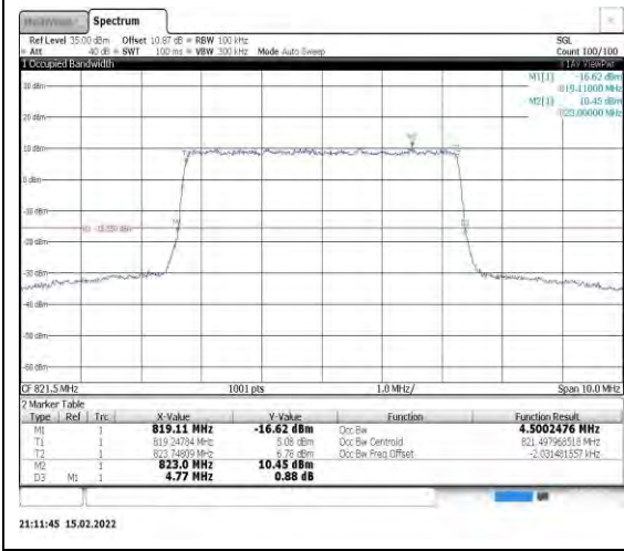
Band26-5MHz-16QAM-26765-25RB#0
