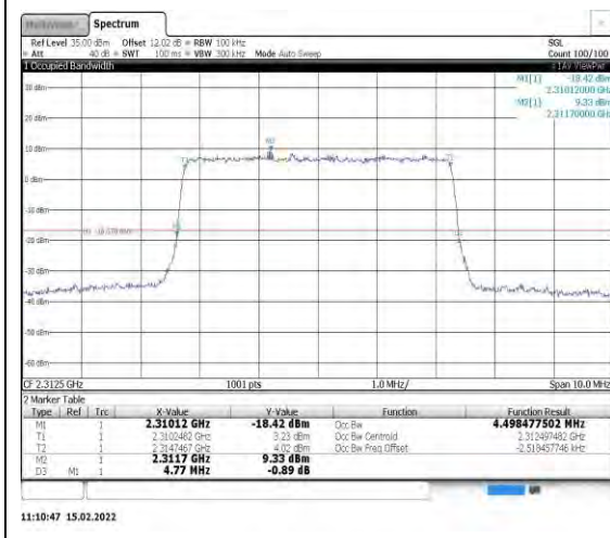
Band40-5MHz-16QAM-38775-25RB#0
