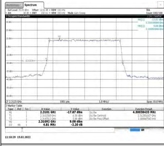
Band40-5MHz-QPSK-38775-25RB#0
