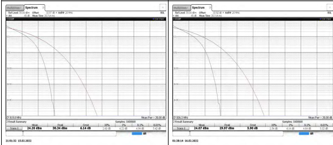
Band26-3MHz-QPSK-26740-15RB#0
