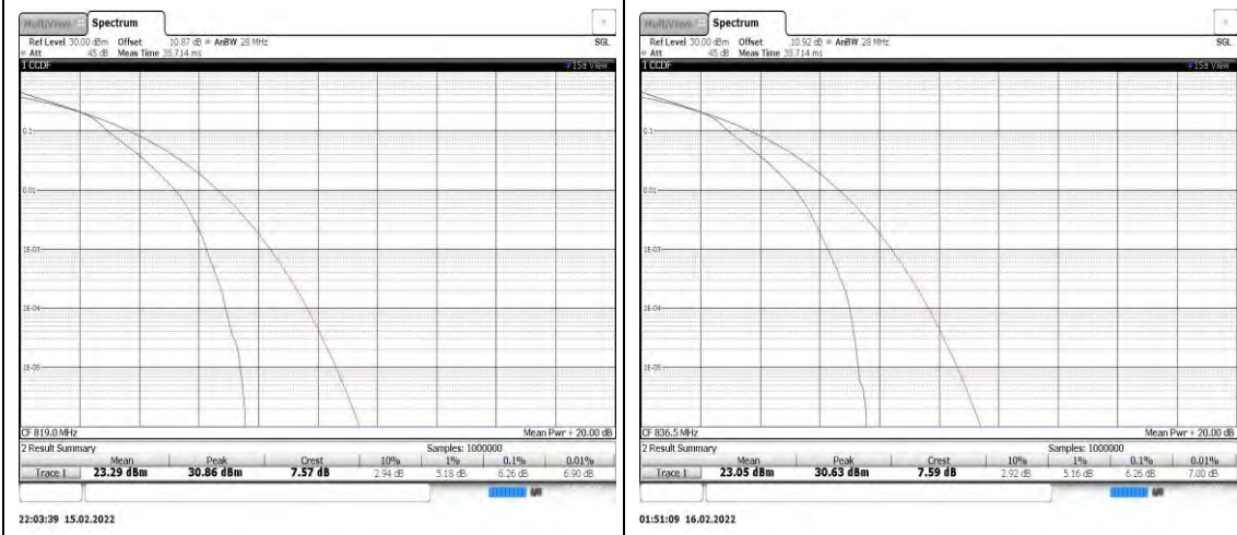
Band26-5MHz-QPSK-26740-25RB#0
