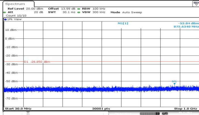
3DH5_Ant1_2441_0~Reference
