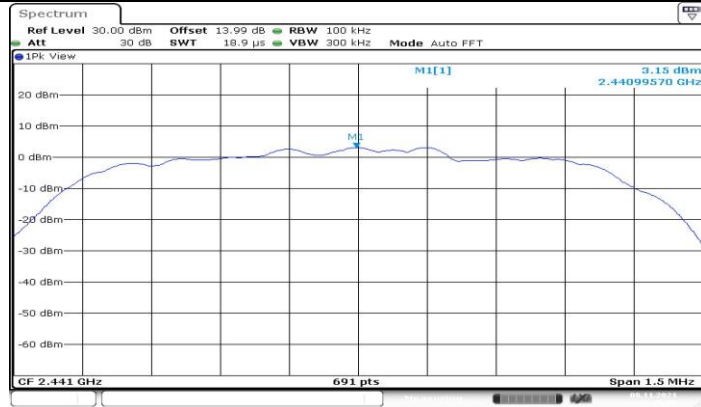
3DH5_Ant1_2441_0~Reference
