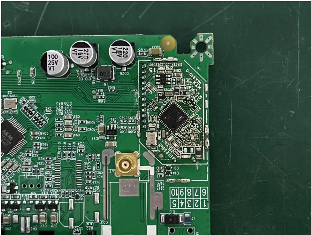
Internal photos M/N: DMX4710S
