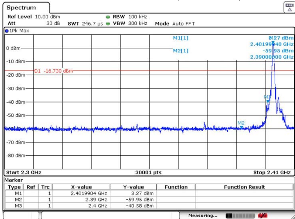
Test Mode: GFSK 2402MHz (NO HOPPING)
