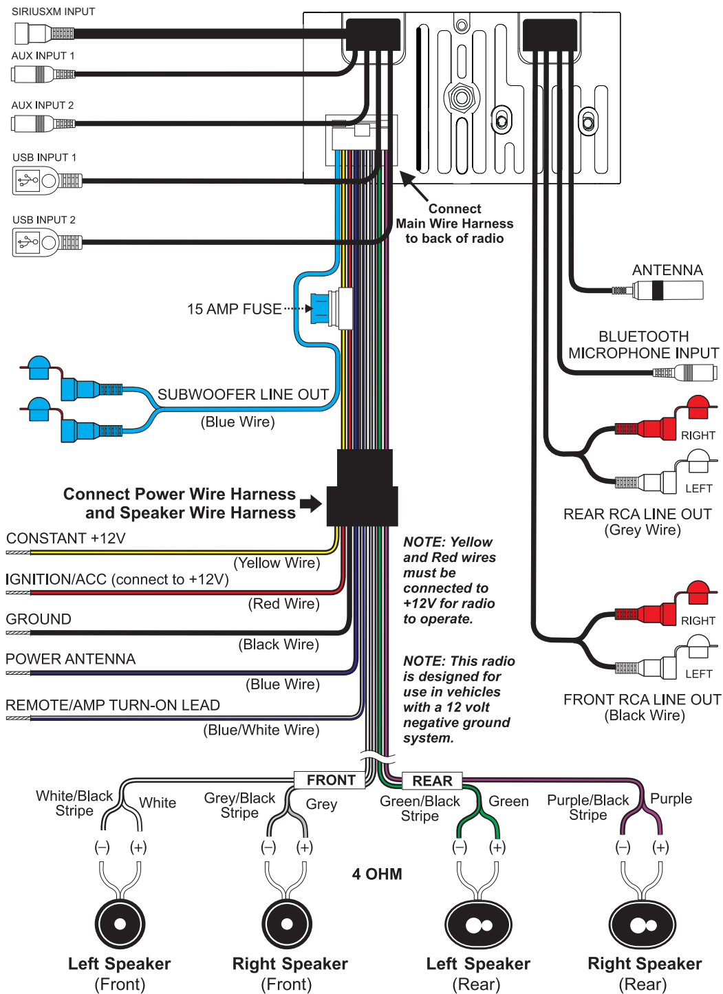
Figure 5 - Wiring Diagram
