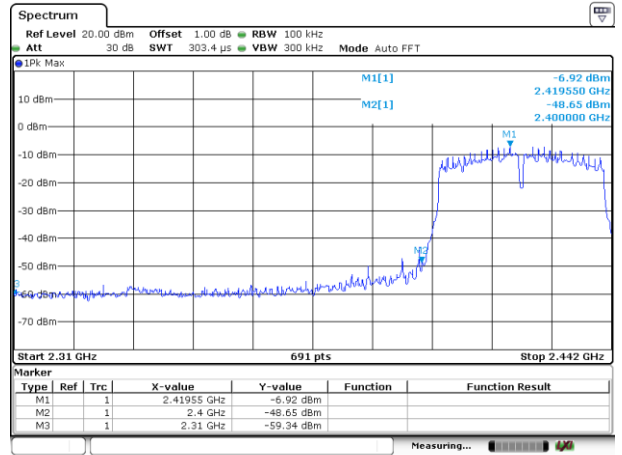
CH03-Bandedge
