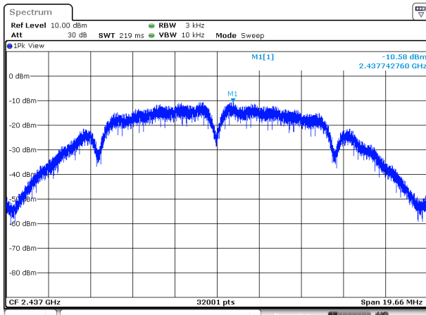
(802.11b) PSD plot on channel 6
