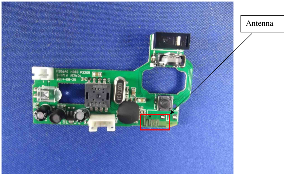
Figure 10 PCB of the EUT-Module View
