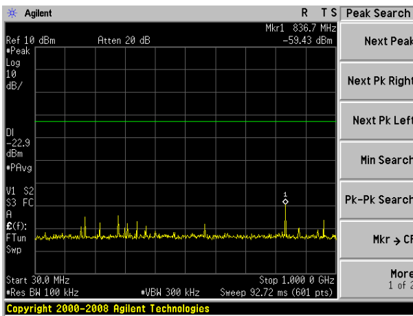
GFSK on channel 04
