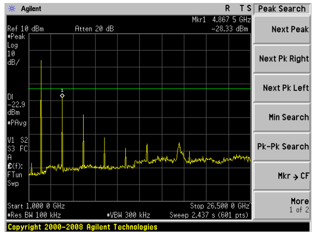
GFSK on channel 04
