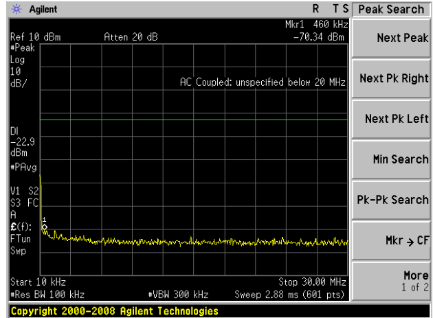
GFSK on channel 04
