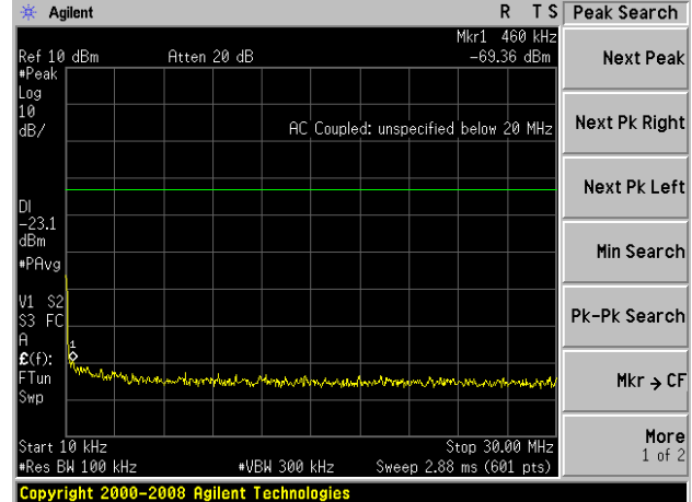
GFSK on channel 08
