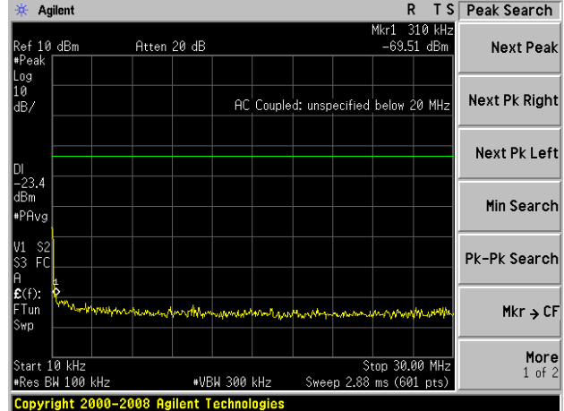
GFSK on channel 01
