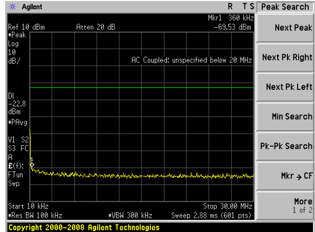
GFSK on channel 04
