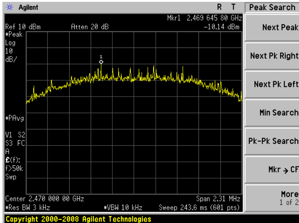
Power spectral density plot on channel 08
