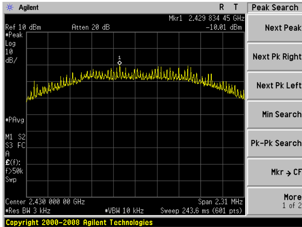
Power spectral density plot on channel 04
