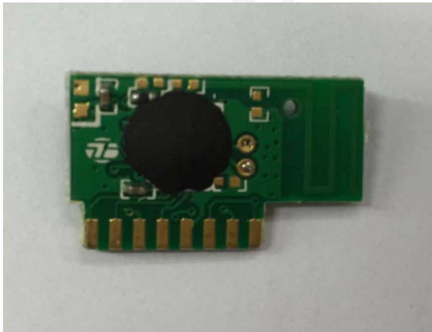
EUT –RF Module Board Top and Antenna View
