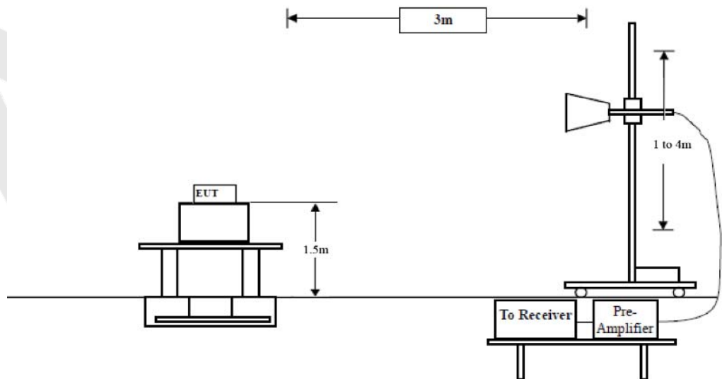
Figure 3. Above 1 GHz
