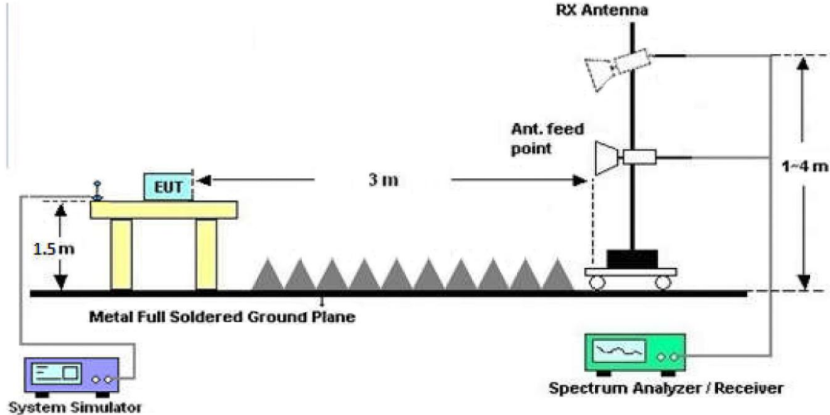
Figure 3. Above 1 GHz
