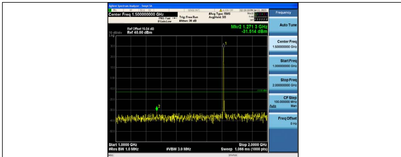
Band4-3MHz-16QAM-19965-1RB#0-Range5:2000~20000MHz
