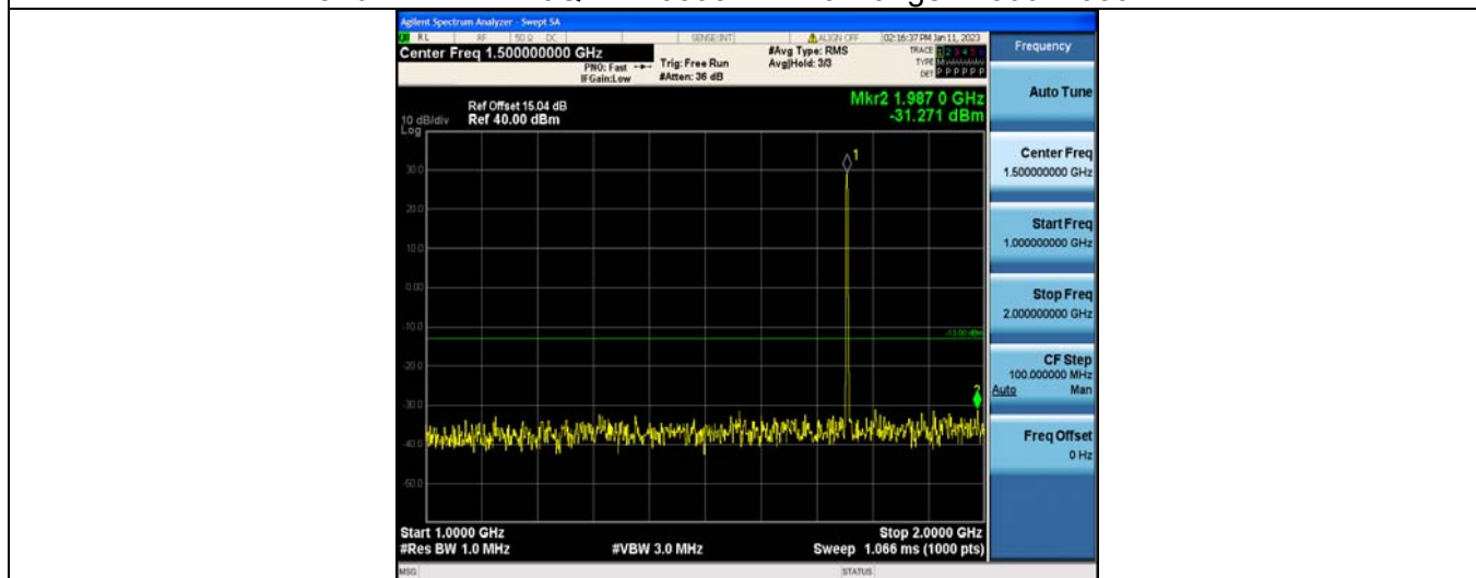
Band4-1.4MHz-16QAM-20393-1RB#0-Range5:2000~20000MHz
