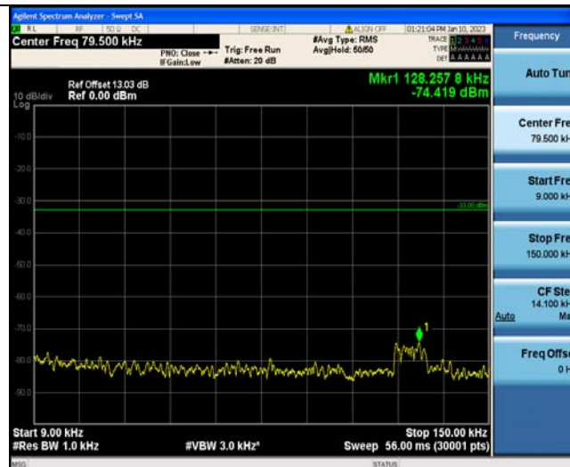
Band5-4132-2-0.009~0.15MHz
