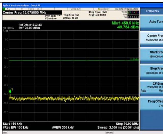
Band5-4183-1-0.15~30MHz
