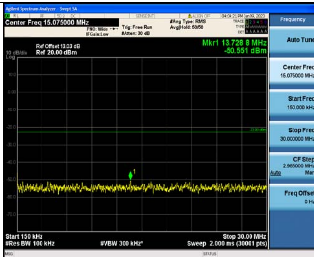
Band2-9538-1-0.15~30MHz
