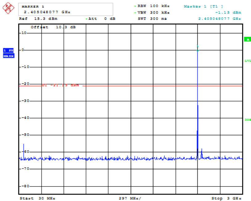
Low Channel 30 MHz – 3 GHz
