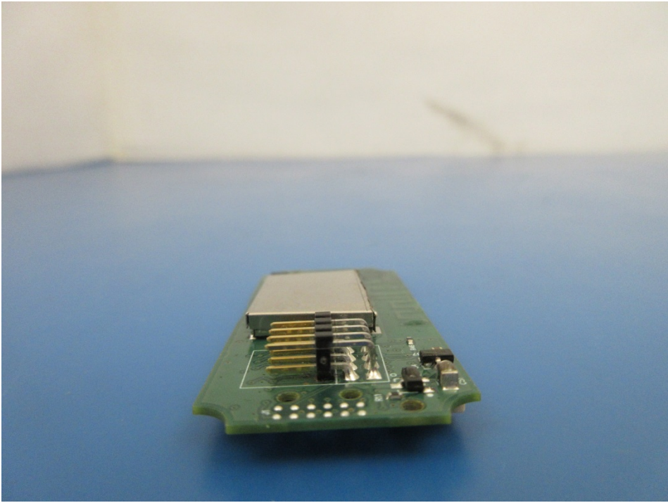
1.8 EUT Bottom Side Right View
