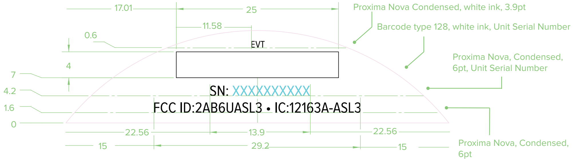
ARTWORK LAYOUT, SCALE 3:1
