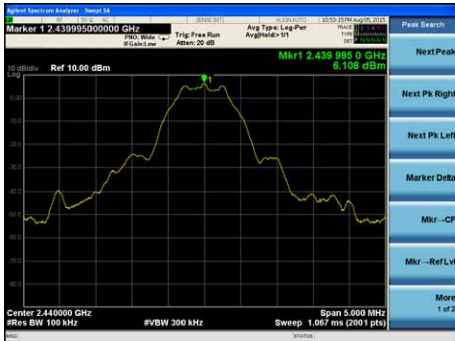
Channel 19 (2440MHz)
