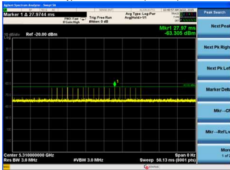
Radar Type 0 Calibration Plot (5310MHz)
