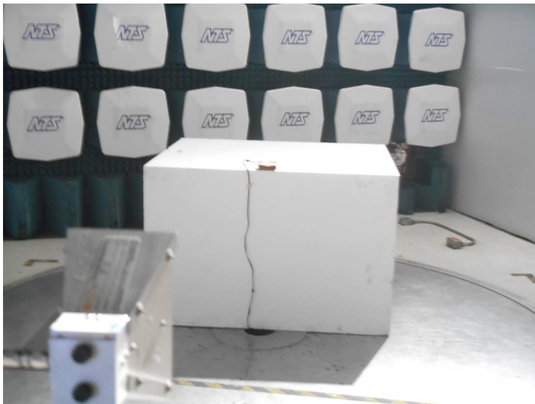
Radiated Emissions (18GHz-25GHz)
