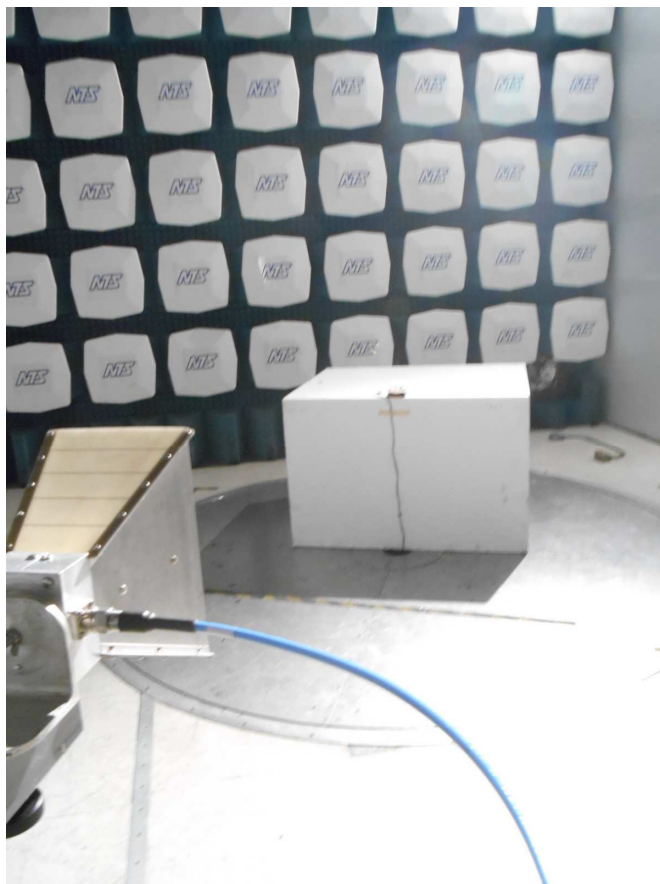
Radiated Emissions (1GHz-18GHz)
