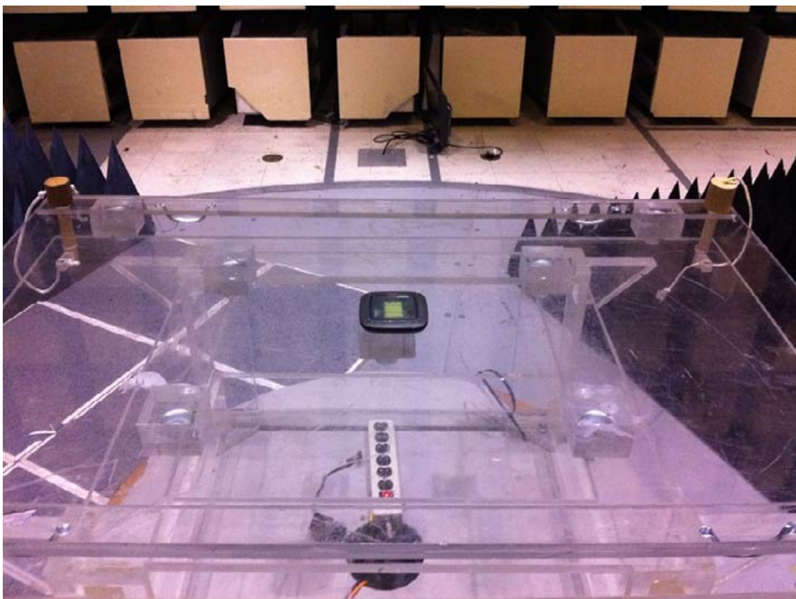
FUNDAMENTAL AND SPURIOUS, FRONT VIEW
