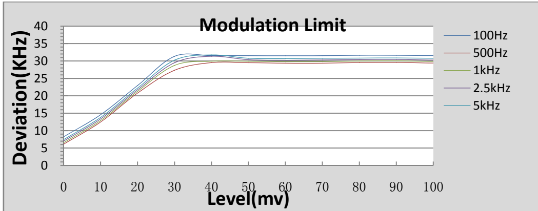
Modulation Deviation of Low Channel
