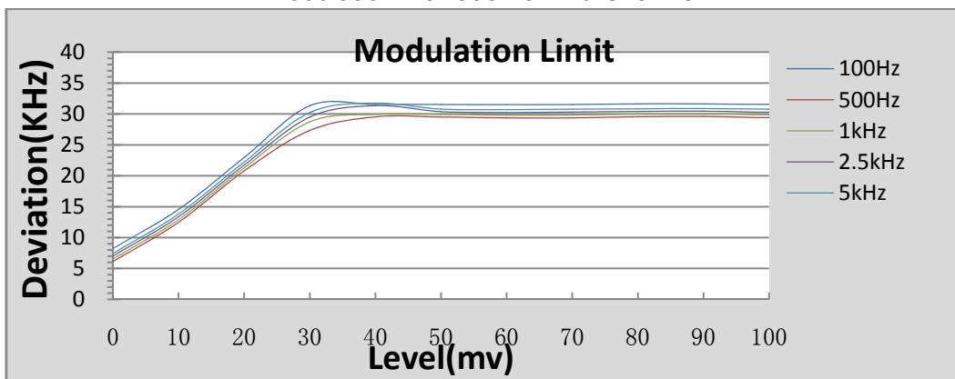
Modulation Deviation of Mid Channel
