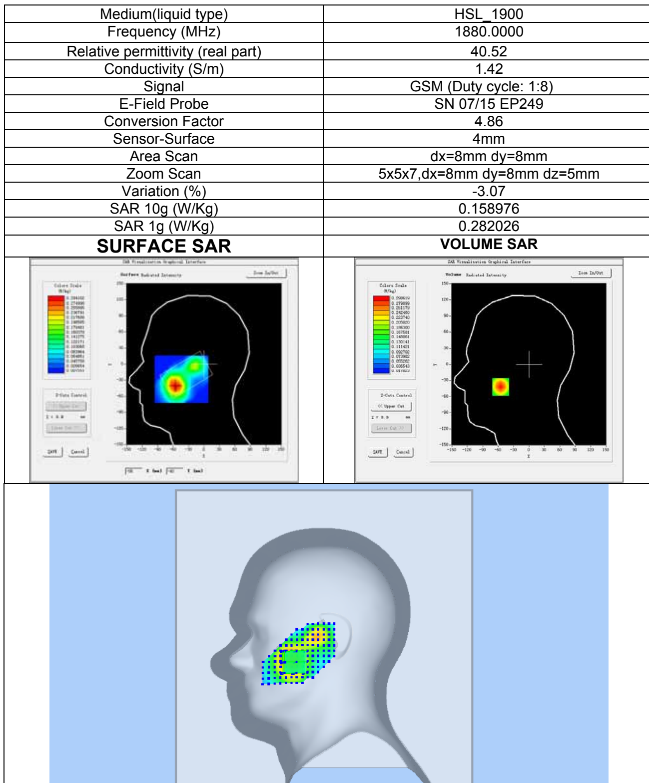
Plot 11: GSM1900, Middle channel (Right Head, Tilt) Product Description: GSM Mobile Phone Test Date: May 22,2017
