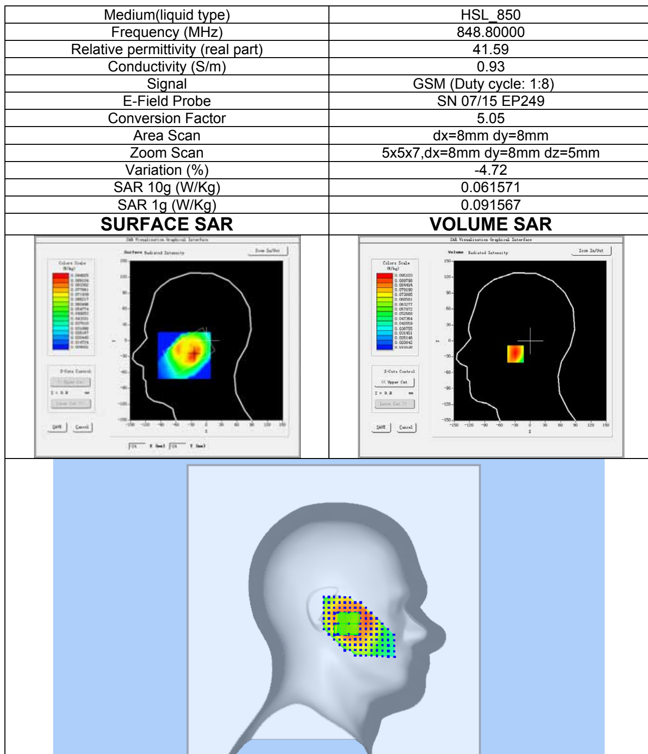
Plot 4: GSM850MHz, High channel (Left Head , Tilt) Product Description: GSM Mobile Phone Test Date:Jul 24,2017
