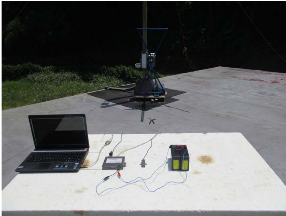
Front View of Mode 1 (with Rectangular Antenna)
