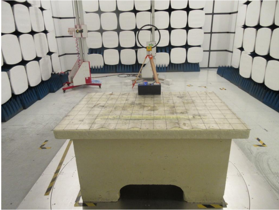
Radiated emission Measurement Photos(9KHz-30MHz)
