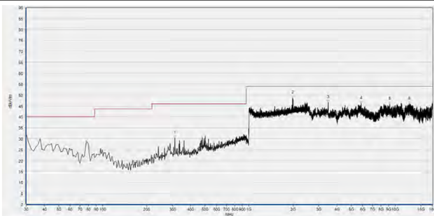
(30MHz to 18GHz, Antenna Horizontal, GFSK, channel 0)
