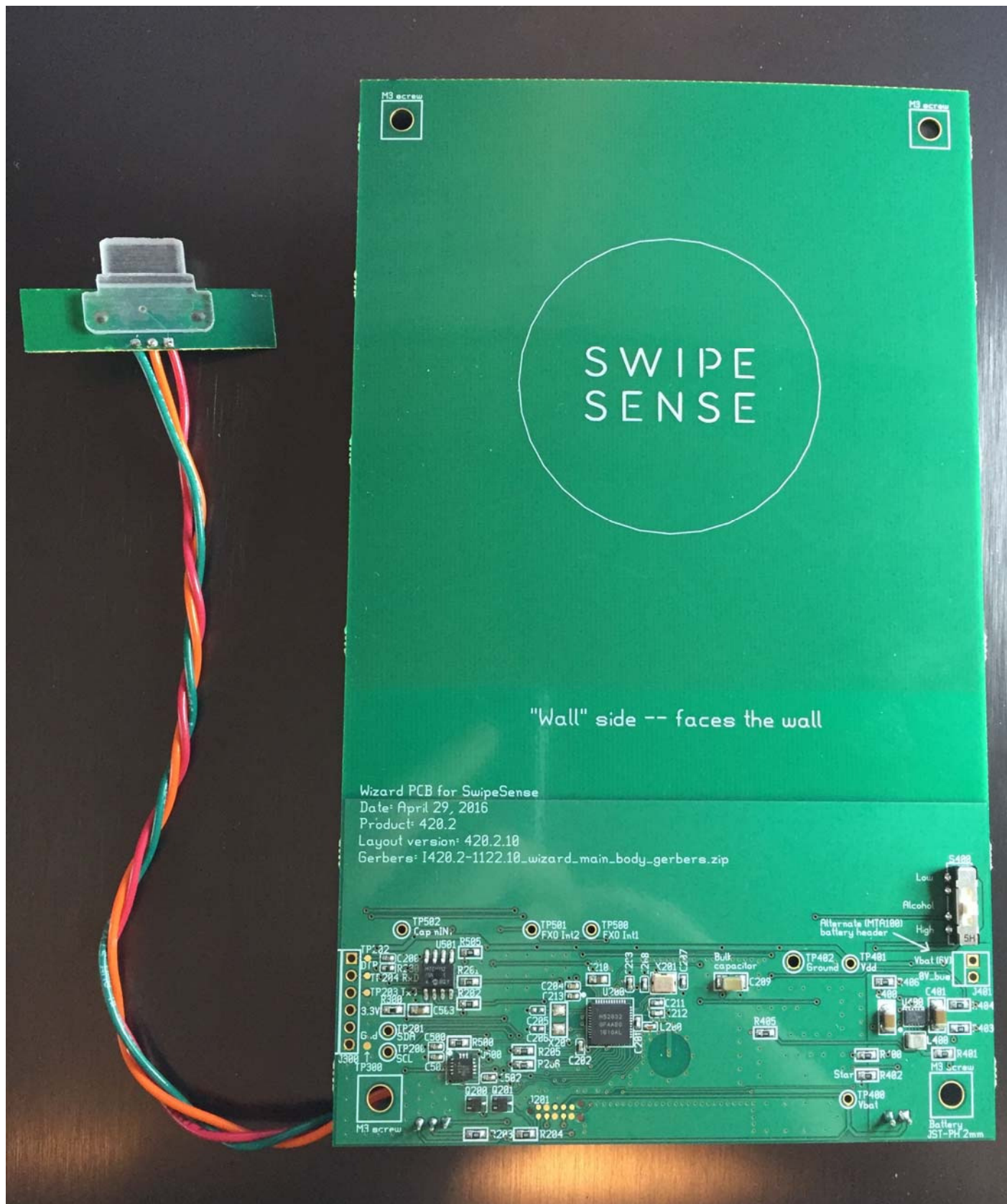
Figure 1 - SwipeSense Hygiene Sensor PWB top view
