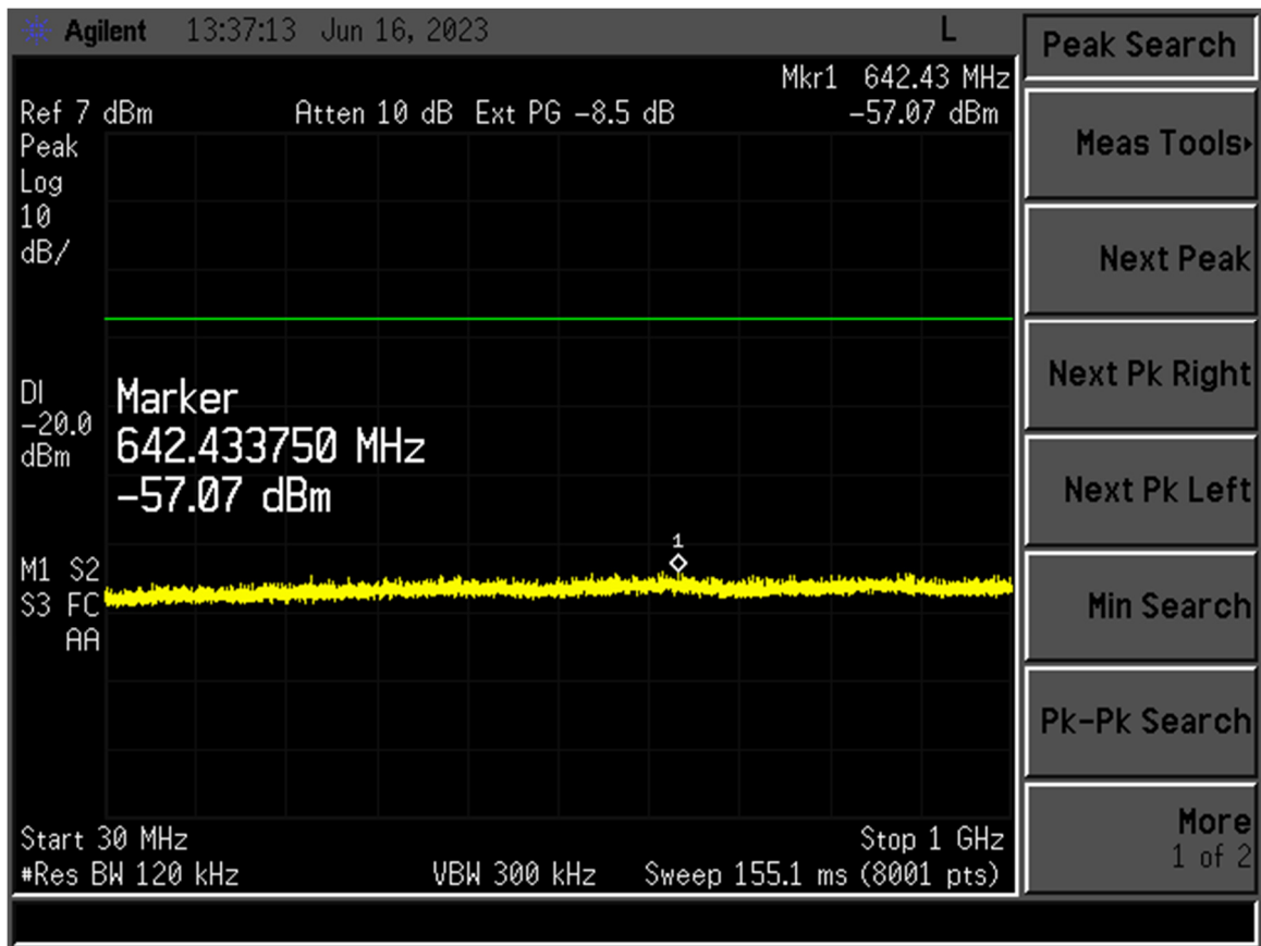
Figure 4. Channel 20, 30-1000 MHz
