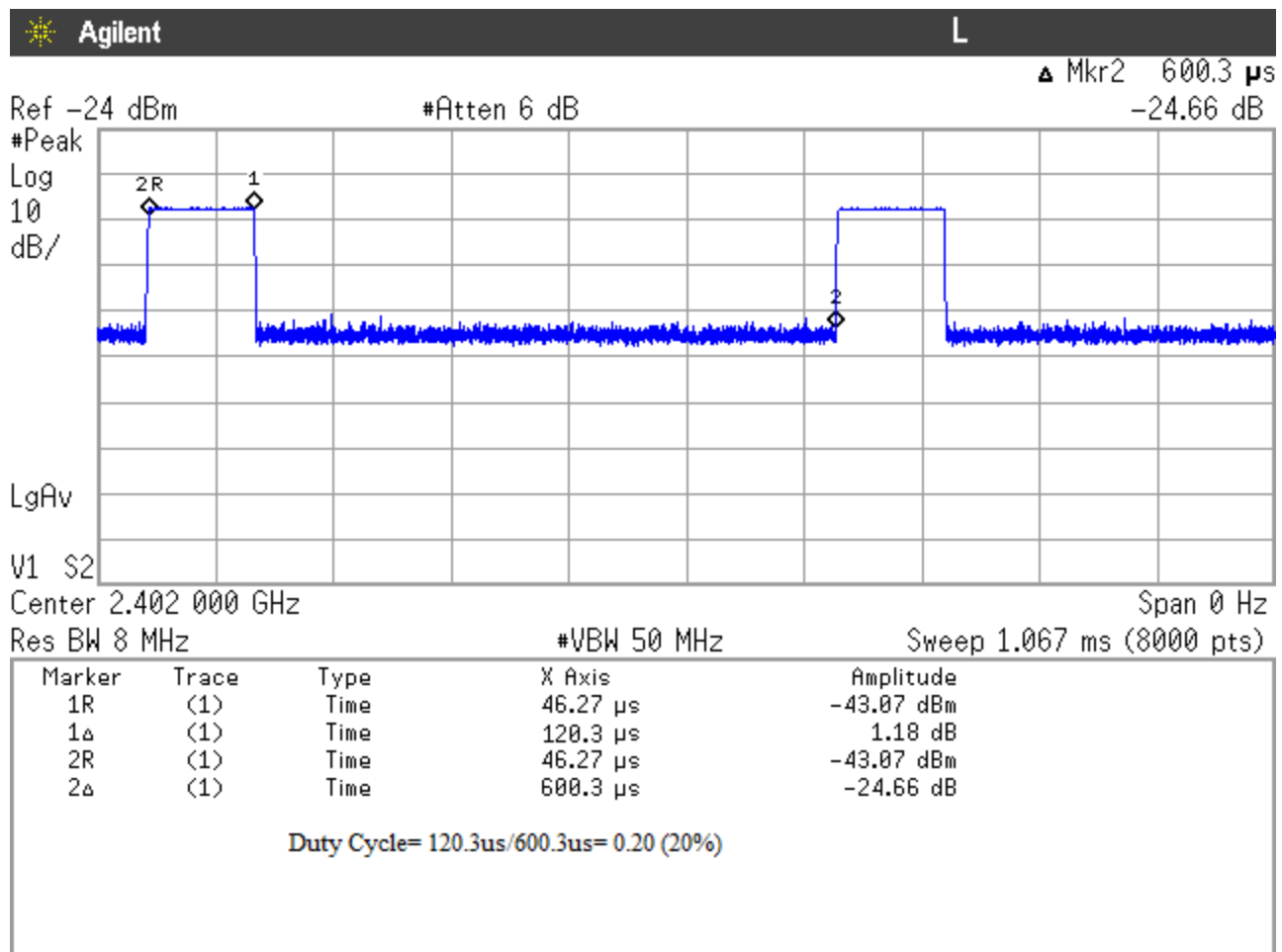
Figure 58: Duty Cycle Calculations
