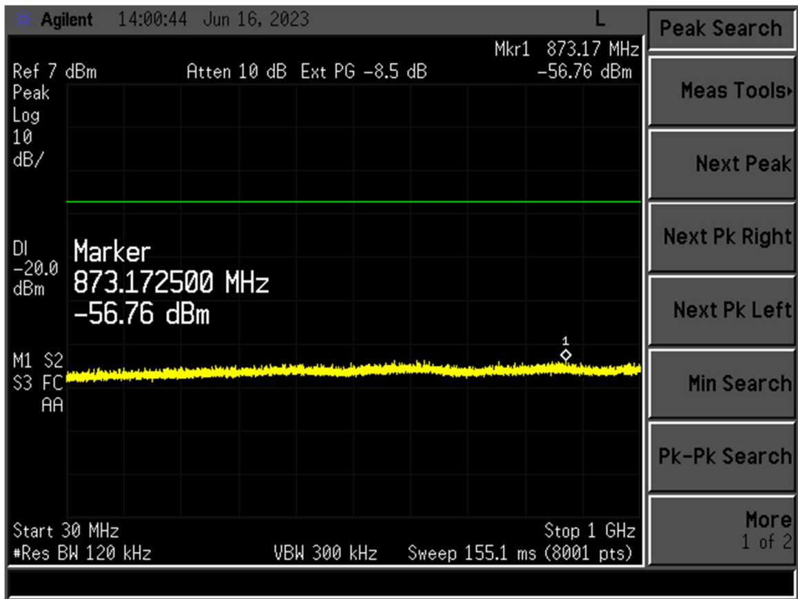
Figure 2. Channel 0, 30-1000 MHz
