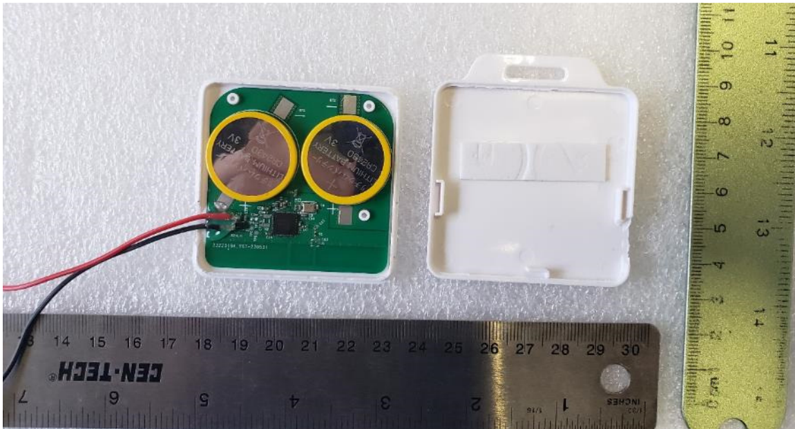
Figure 1. EUT, Front Cover Removed
