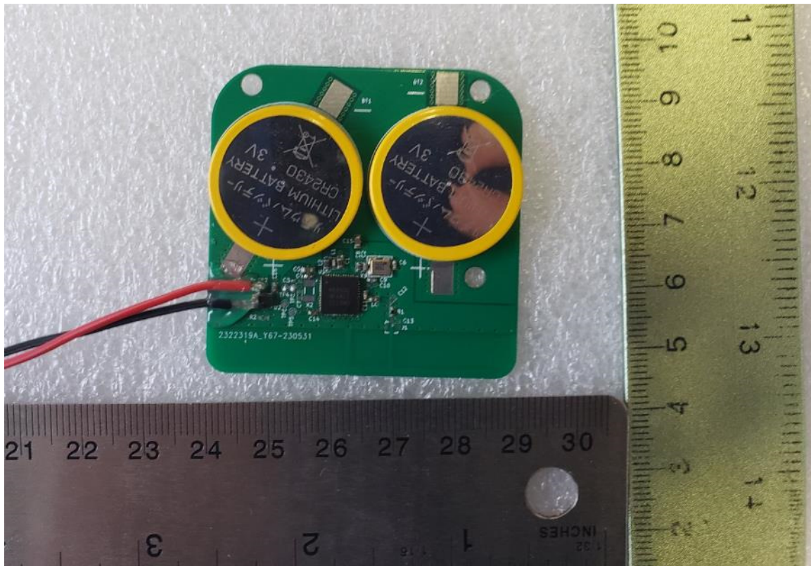
Figure 3. Front of Main PCB
