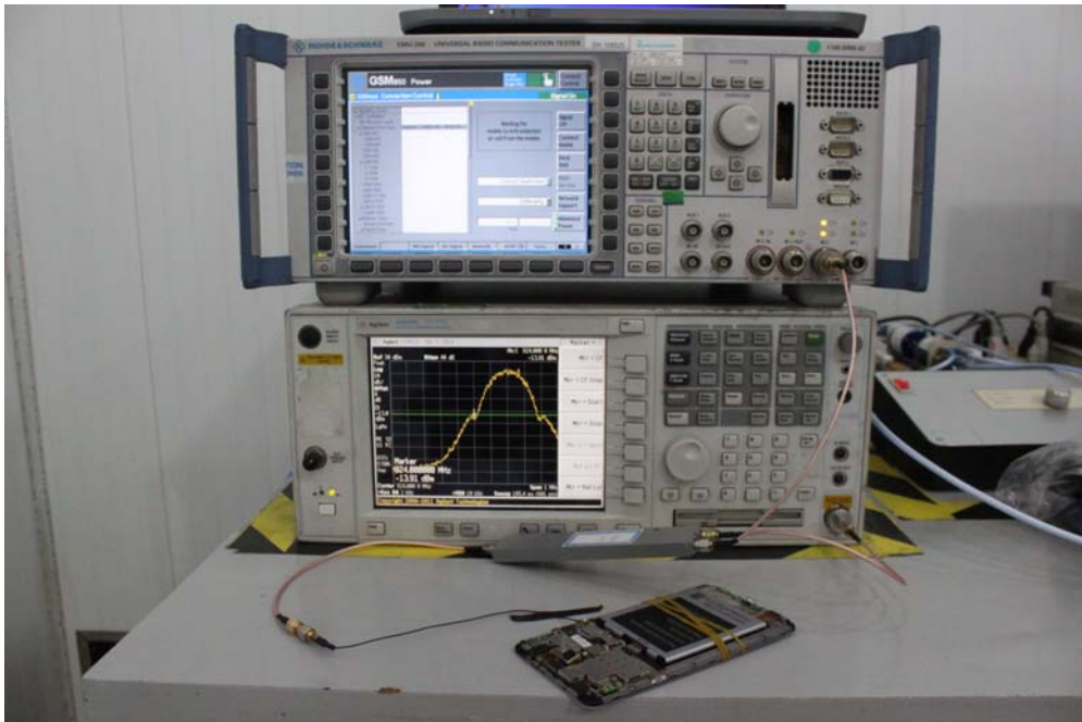
Conducted Test
