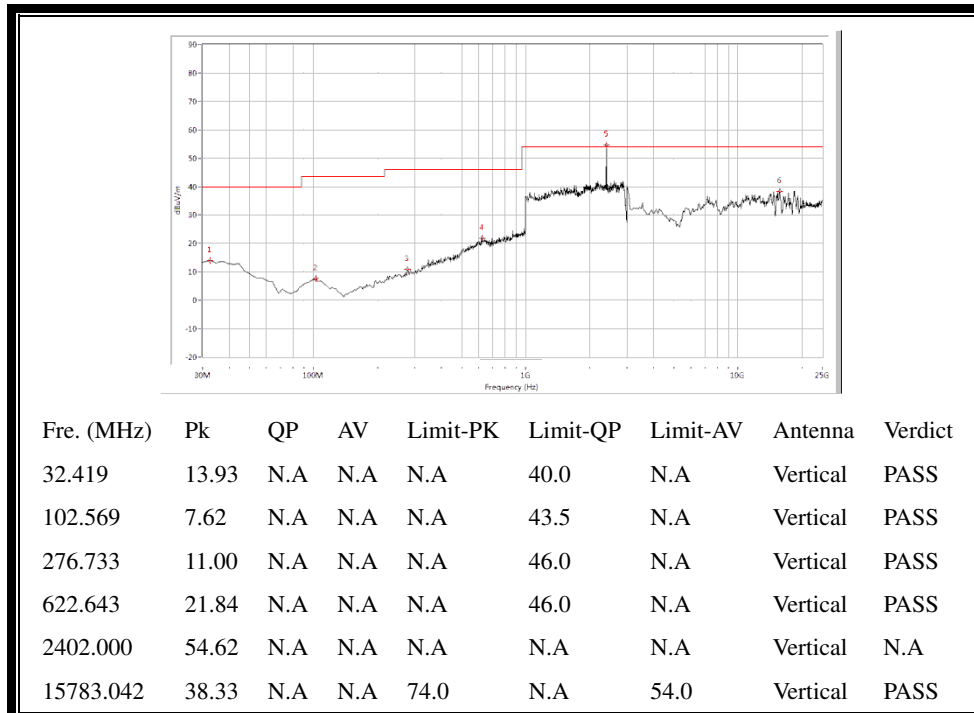
(30MHz to 25GHz, Antenna Vertical @ \pi/4 -DQPSK, channel 0)
