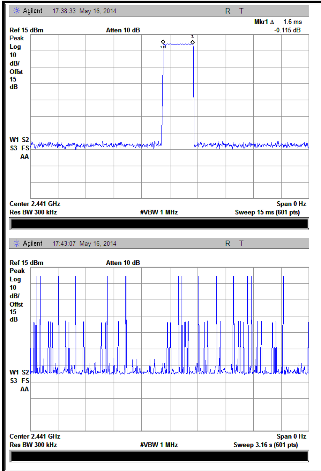
(Plot E: DH3 @ 1/4-DQPSK)
