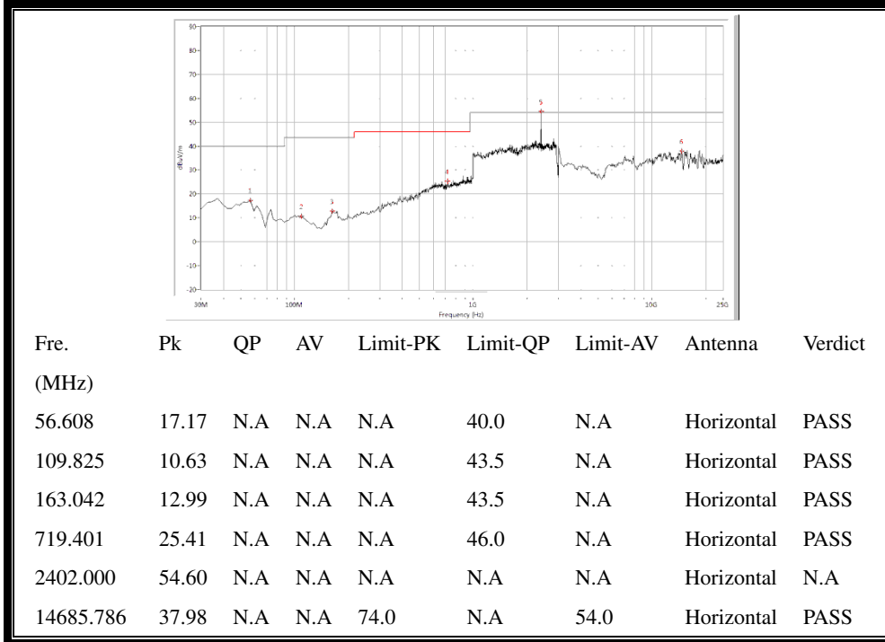
(30MHz to 25GHz, Antenna Horizontal @ \pi/4 -DQPSK, channel 0)
