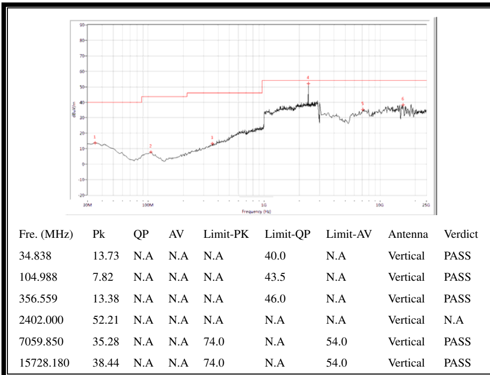
(30MHz to 25GHz, Antenna Vertical @ GFSK, channel 0)
