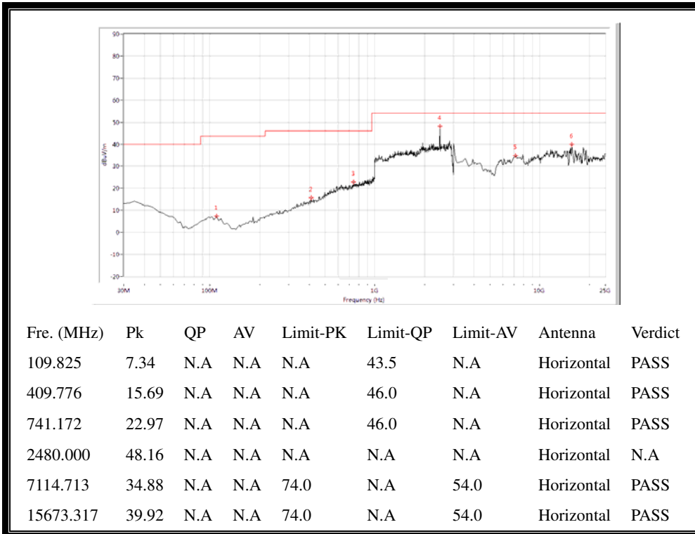
(30MHz to 25GHz, Antenna Horizontal @8-DPSK, channel 78)
