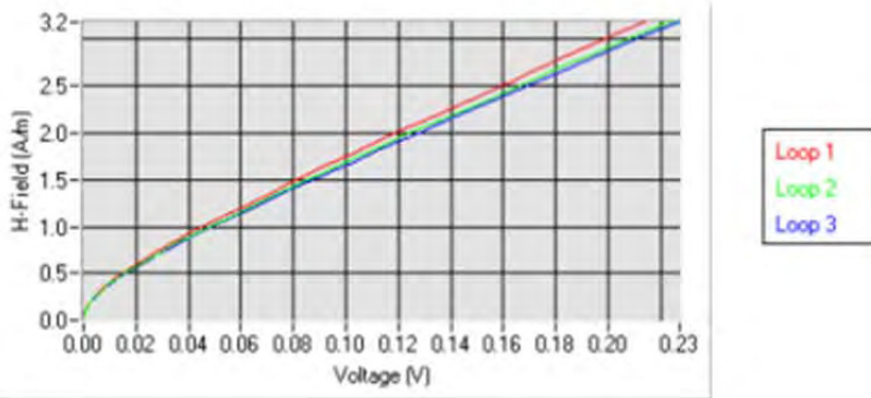
Calibration curves at 835 MHz
