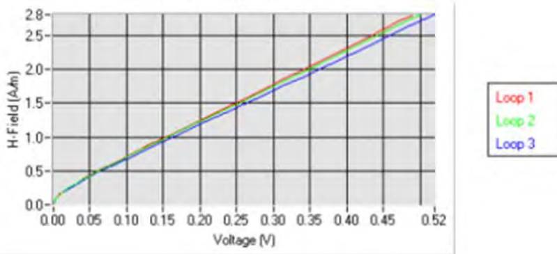
Calibration curves at 1900 MHz
