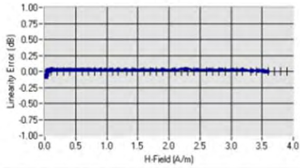
Linearity
