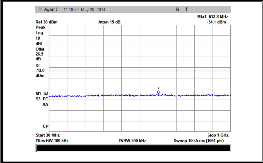
(Plot D: CDMA 1900MHz:BC 1 Channel = 25, 30MHz to 1GHz)
