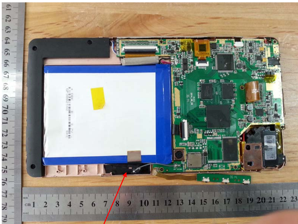
WIFI/BT Antenna
