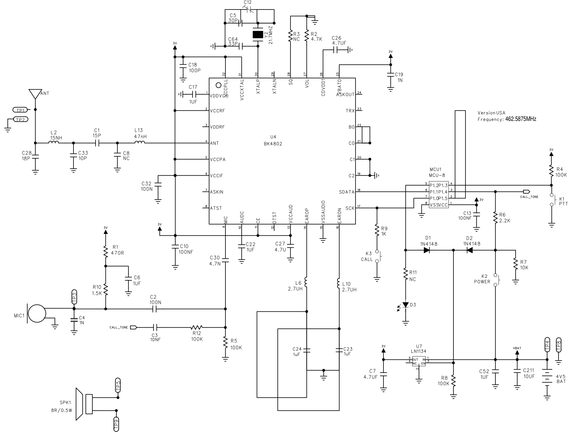
10526 Walkie talkie schematic diagram
