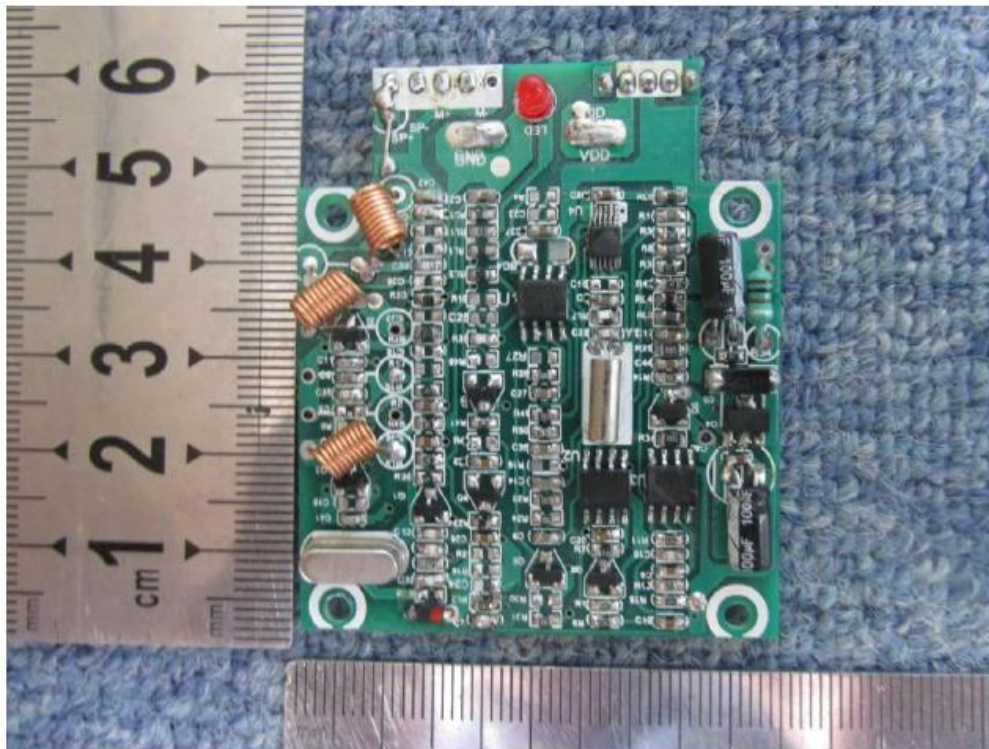
Ear Bud Receiver Main Board Top View
