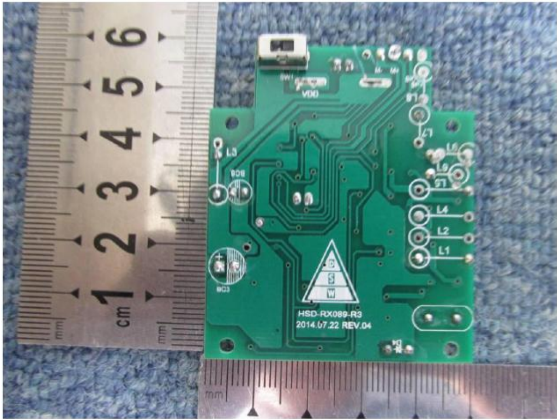
Ear Bud Receiver Main Board Bottom View
