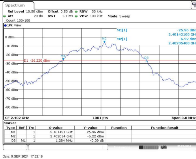
2DH5_Ant1_2402
