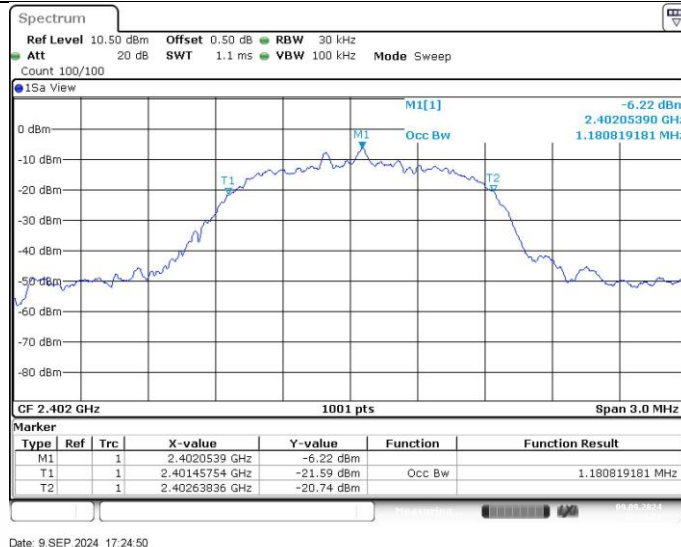
3DH5_Ant1_2402
