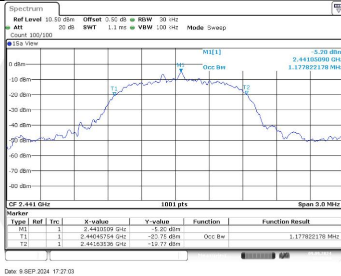
3DH5_Ant1_2441
