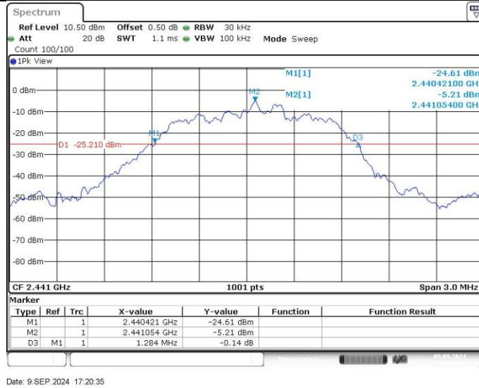
2DH5_Ant1_2441
