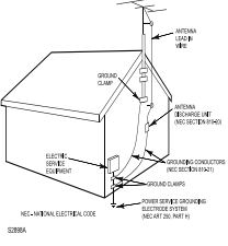
EXAMPLE OF ANTENNA GROUNDING AS PER NATIONAL ELECTRICAL CODE
