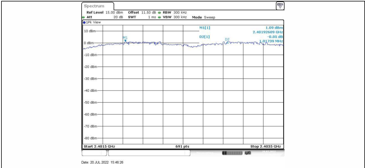
3DH5_Ant1_Hop_2441
