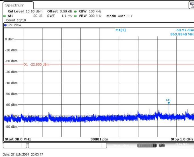
DH5_Ant1_2402_30~1000
