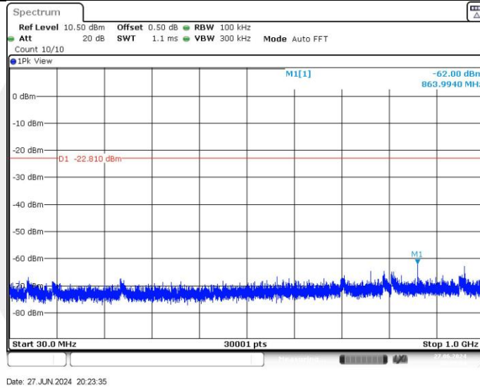
3DH5_Ant1_2480_30~1000
