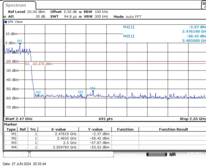
2DH5_Ant1_High_Hop_2480
