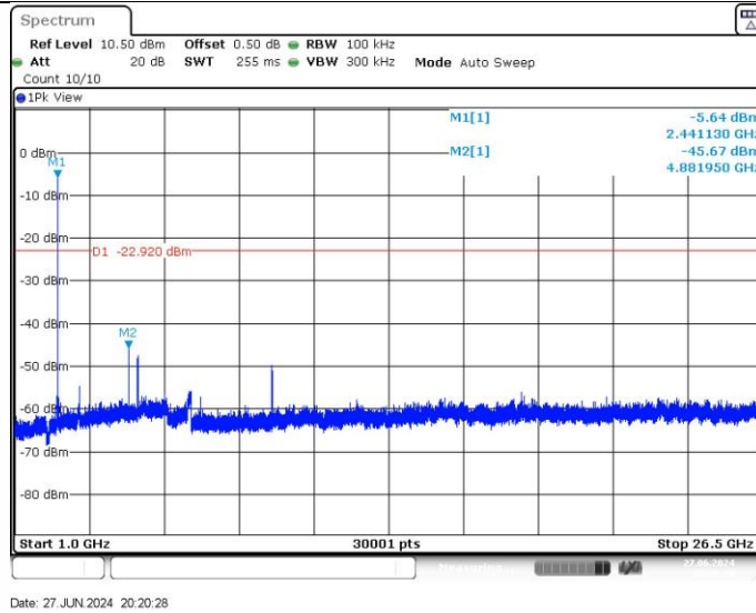
3DH5_Ant1_2441_1000~26500
