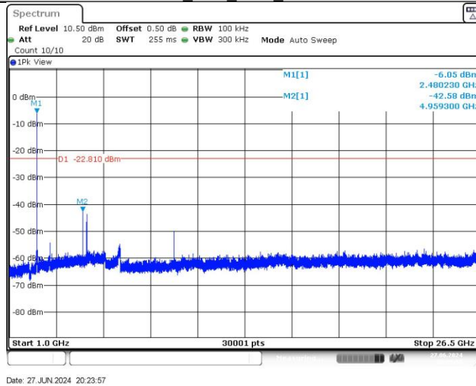
3DH5_Ant1_2480_1000~26500
