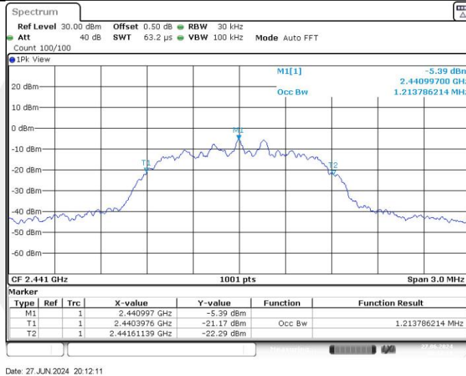
2DH5_Ant1_2441
